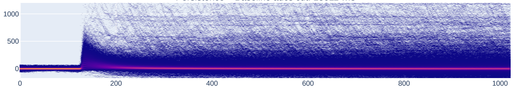
Persistence – Baseline adcs cut: 13611 wfs
