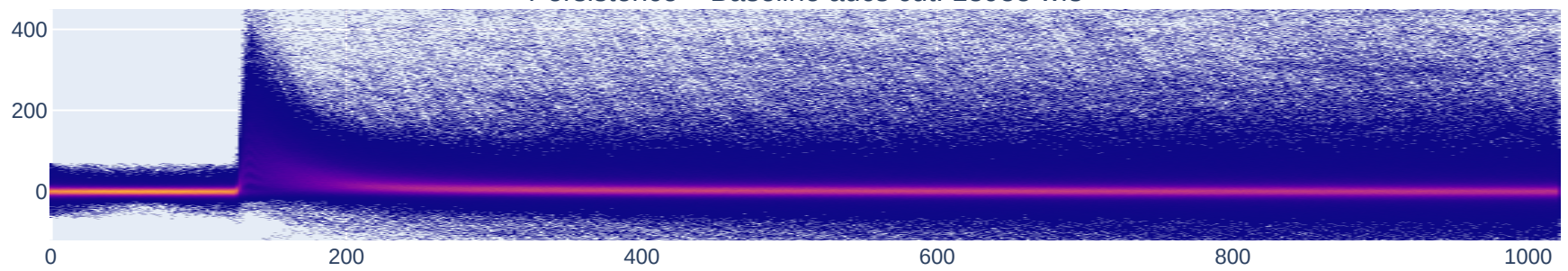
Persistence – Baseline adcs cut: 13955 wfs
