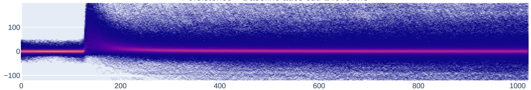
Persistence – Baseline adcs cut: 14075 wfs
