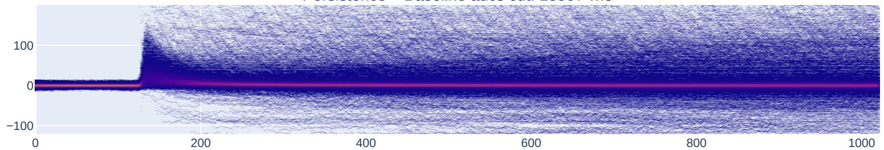
Persistence – Baseline adcs cut: 13507 wfs
