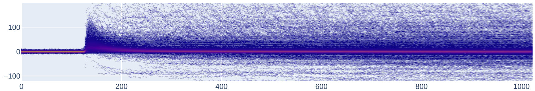
Persistence – Baseline std cut: 10472 wfs
