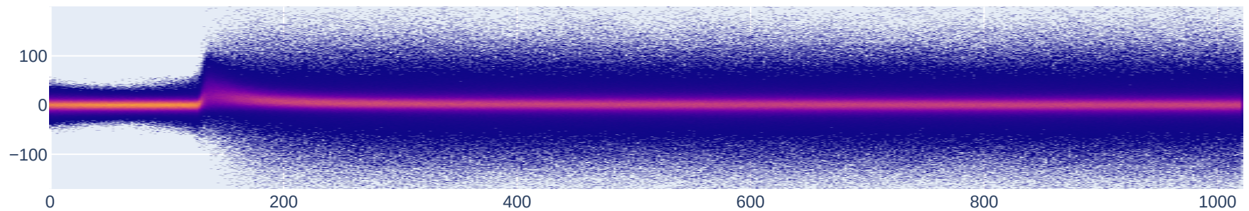
Persistence – Baseline std cut: 10208 wfs
