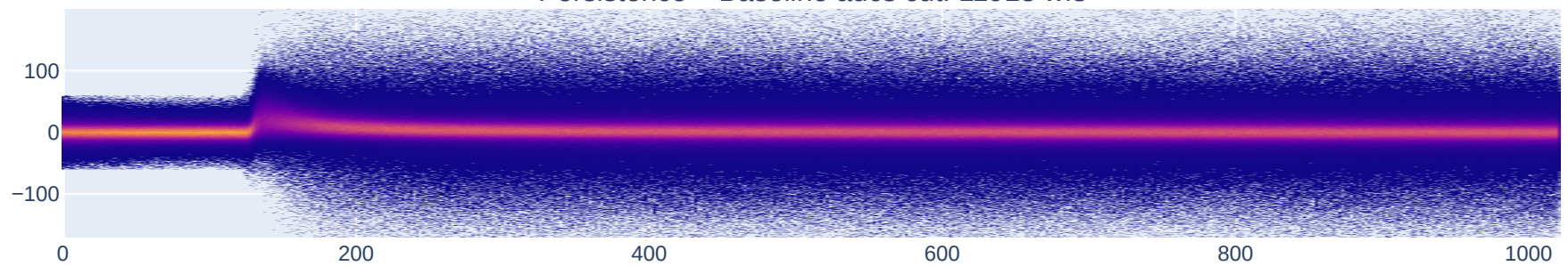
Persistence – Baseline adcs cut: 11918 wfs
