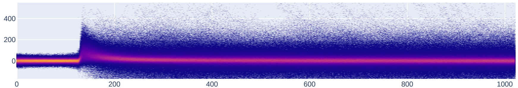
Persistence – Baseline std cut: 7392 wfs
