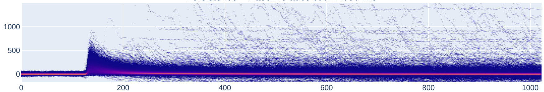
Persistence – Baseline adcs cut: 14600 wfs
