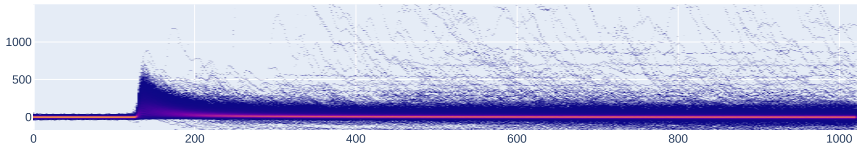
Persistence – Baseline std cut: 12415 wfs
