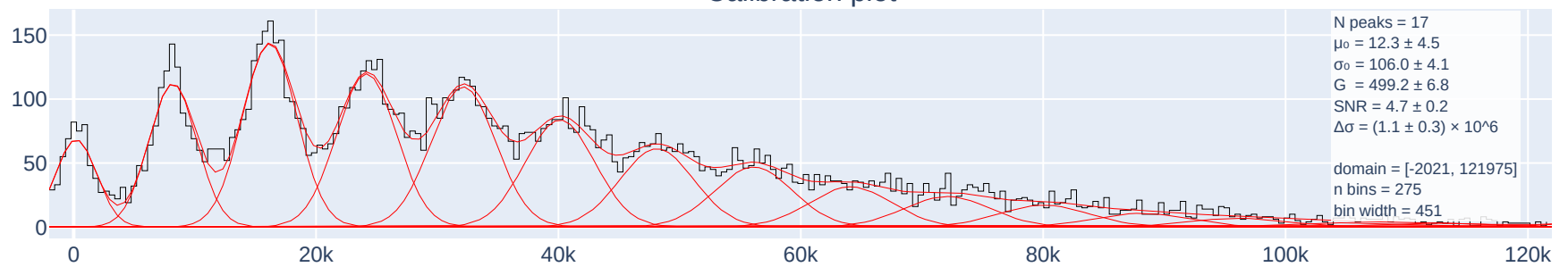
Calibration plot
