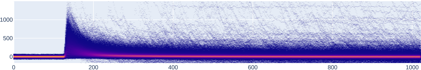
Persistence – Baseline std cut: 11663 wfs
