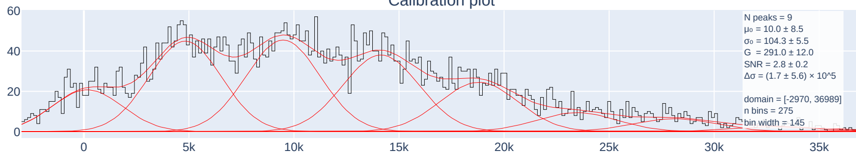
Calibration plot
