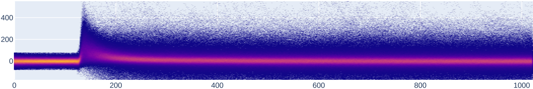
Persistence – Baseline adcs cut: 8258 wfs
