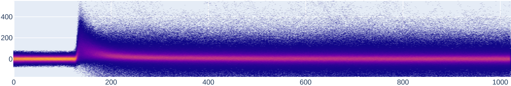
Persistence – Baseline std cut: 6849 wfs
