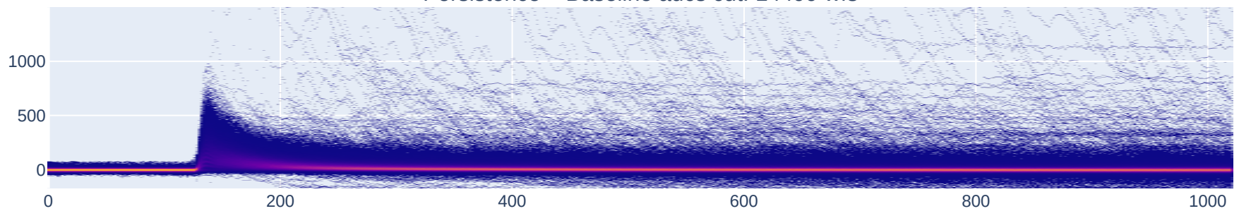
Persistence – Baseline adcs cut: 14499 wfs
