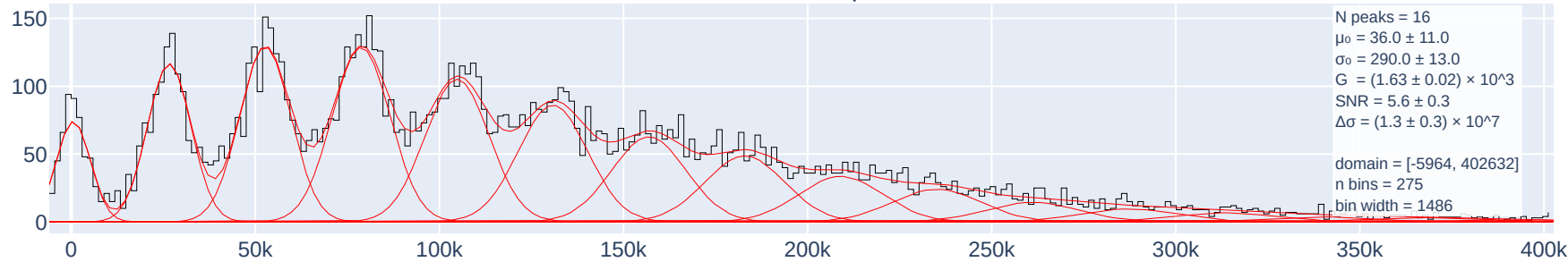
Calibration plot
