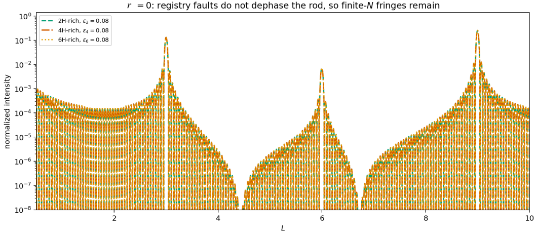
Figure S4: Calculation-only check of the phase-insensitive r = 0 condition. Different parent-rich transition laws coincide because registry and orientation changes do not alter the local 00L amplitude. The remaining oscillations are controlled by finite stack length.
