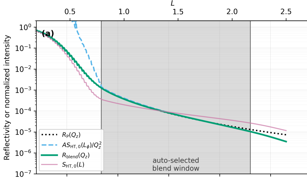
Figure 7: Optical-to-structural handoff used for the near-critical specular-family calculation. (a) Pure Parratt reflectivity gives the low- Q_z optical response, including refraction, evanescence, and multiple reflection at the film interfaces. The high- Q_z branch is the normalized finite-stack structure term divided by Q_z^2 and scaled to the optical branch in an overlap region. The final curve is a smooth log-intensity blend between these limits, plotted versus Q_z/Q_c with the corresponding crystallographic L coordinate on the top axis.
