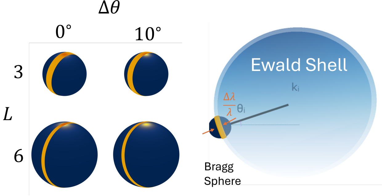
Figure 8: Bandwidth, refraction, and mosaic-cap geometry for the low- L m = 0 feature. The wavelength distribution changes both the Ewald-sphere radius and the refractive index used to calculate the internal wavevector. Because G_{00L} \propto L , a fixed bandwidth samples a larger angular fraction of low- L Bragg spheres than high- L Bragg spheres.
