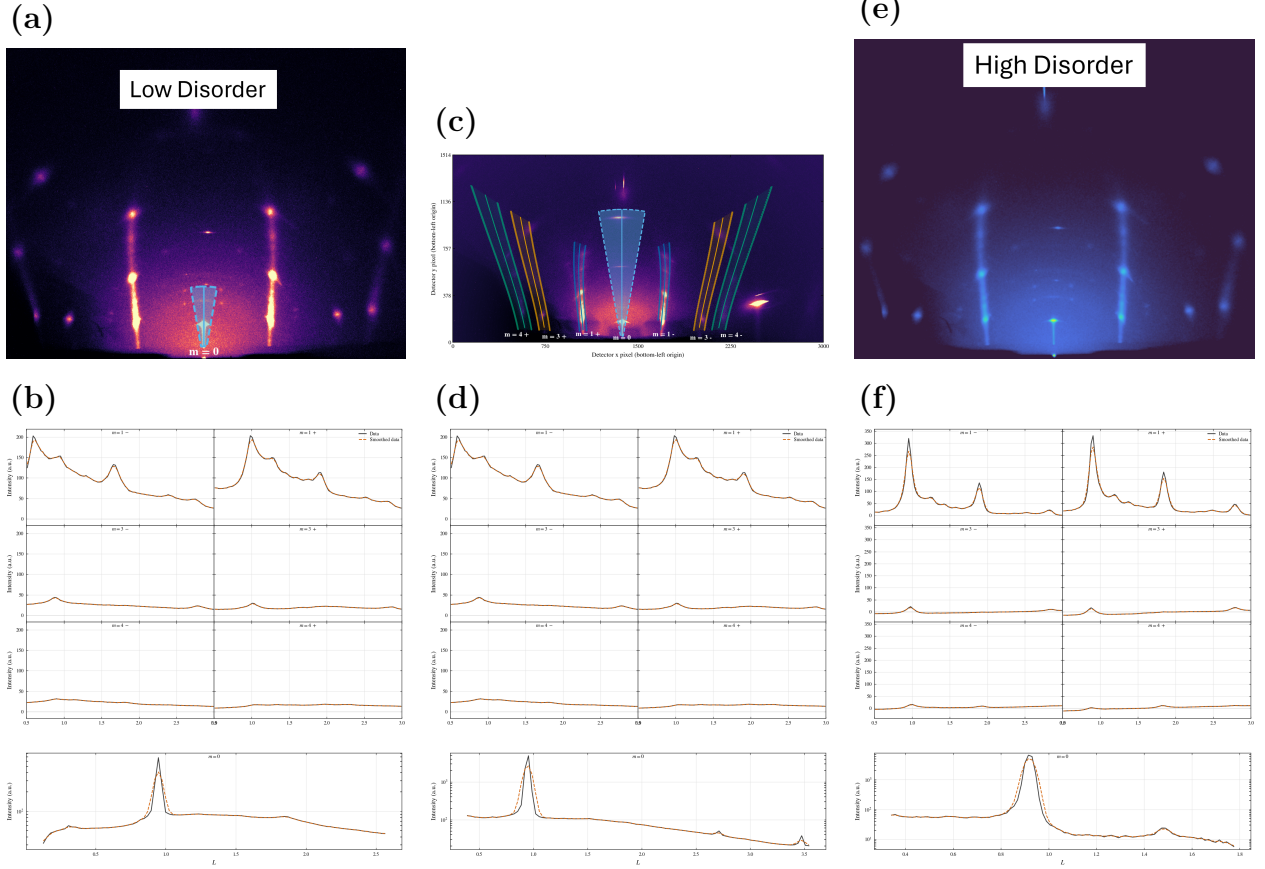
Figure 11: \text{PbI}_2 diffuse-rod validation at \theta_i = 4^\circ for samples spanning increasing stacking disorder. The left column, (a,b), shows a less-disordered sample with prominent peaks. The middle column, (c,d), shows a sample with intermediate disorder seen from the diffuse between the peaks. The right column, (e,f), shows a highly disordered sample with pronounced stacking faults. In the top row, measured detector images are shown with selected constant- m extraction regions overlaid. Solid colored curves mark the projected rod centerlines, semi-transparent regions mark the integrated detector pixels, and dashed outlines mark the integration-band boundaries. The labels m identify two-dimensional powder rod families, with signs distinguishing the two detector-side branches of the same family. In the bottom row, extracted profiles are plotted versus L after applying the same projection to measured and calculated images. Black solid curves are measured data and orange dashed curves are simulations. The progression across the three samples shows how increasing stacking disorder modifies the diffuse-rod profiles while testing the stacking-disorder model, detector geometry, mosaic broadening, and relative structure-factor weighting of the constant- m rod families.
