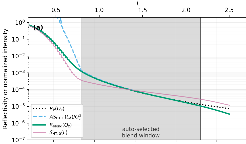
Figure 6: Optical-to-structural handoff used for the near-critical specular-family calculation. (a) Pure Parratt reflectivity gives the low- Q_z optical response, including refraction, evanescence, and multiple reflection at the film interfaces. The high- Q_z branch is the normalized finite-stack structure term divided by Q_z^2 and scaled to the optical branch in an overlap region. The final curve is a smooth log-intensity blend between these limits, plotted versus Q_z/Q_c with the corresponding crystallographic L coordinate on the top axis. Q_z .
