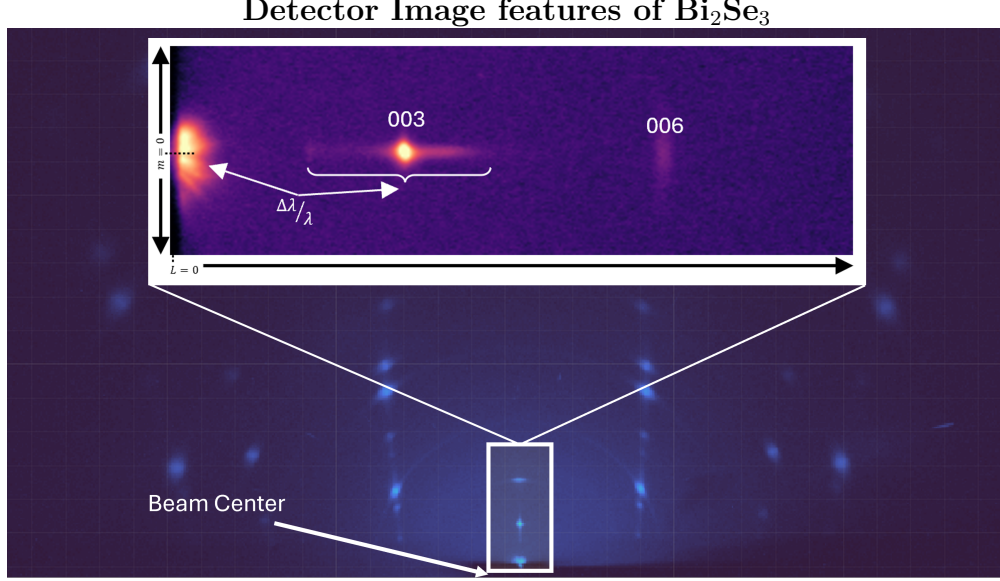
Figure 4: Close-up of the low- L m = 0 detector feature from the 5^\circ \text{Bi}_2\text{Se}_3 . The bright near-origin intensity and vertical star-like morphology are not expected from an ideal single-crystallite calculation or from a mosaic distribution with only a rapidly decaying core. The feature reflects the combined effect of wavelength bandwidth and angular divergence, which give the Ewald sphere an effective thickness, and a long mosaic tail, which supplies tilted crystallites that bring otherwise off-condition specular-family intensity into the measured detector region.
