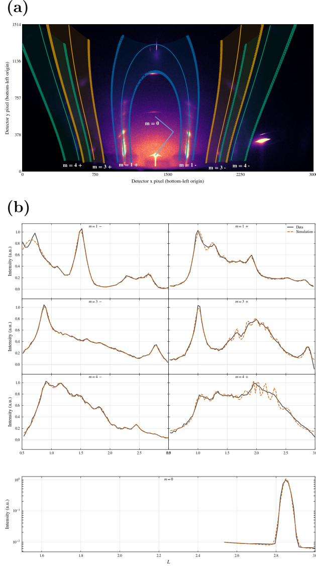
Figure 10: \text{PbI}_2 diffuse-rod validation at \theta_i = 4^\circ . (a) Measured detector image with selected constant- m extraction regions overlaid. Solid colored curves mark the projected rod center-lines, semi-transparent regions mark the integrated detector pixels, and dashed outlines mark the integration-band boundaries. The labels m identify two-dimensional powder rod families, with signs distinguishing the two detector-side branches of the same family. (b) Extracted profiles plotted versus L after applying the same projection to measured and calculated images. Black solid curves are measured data and orange dashed curves are simulations. The agreement across the off-specular diffuse rods tests the stacking-disorder model, detector geometry, mosaic broadening, and the relative structure-factor weighting of the constant- m rod families.
