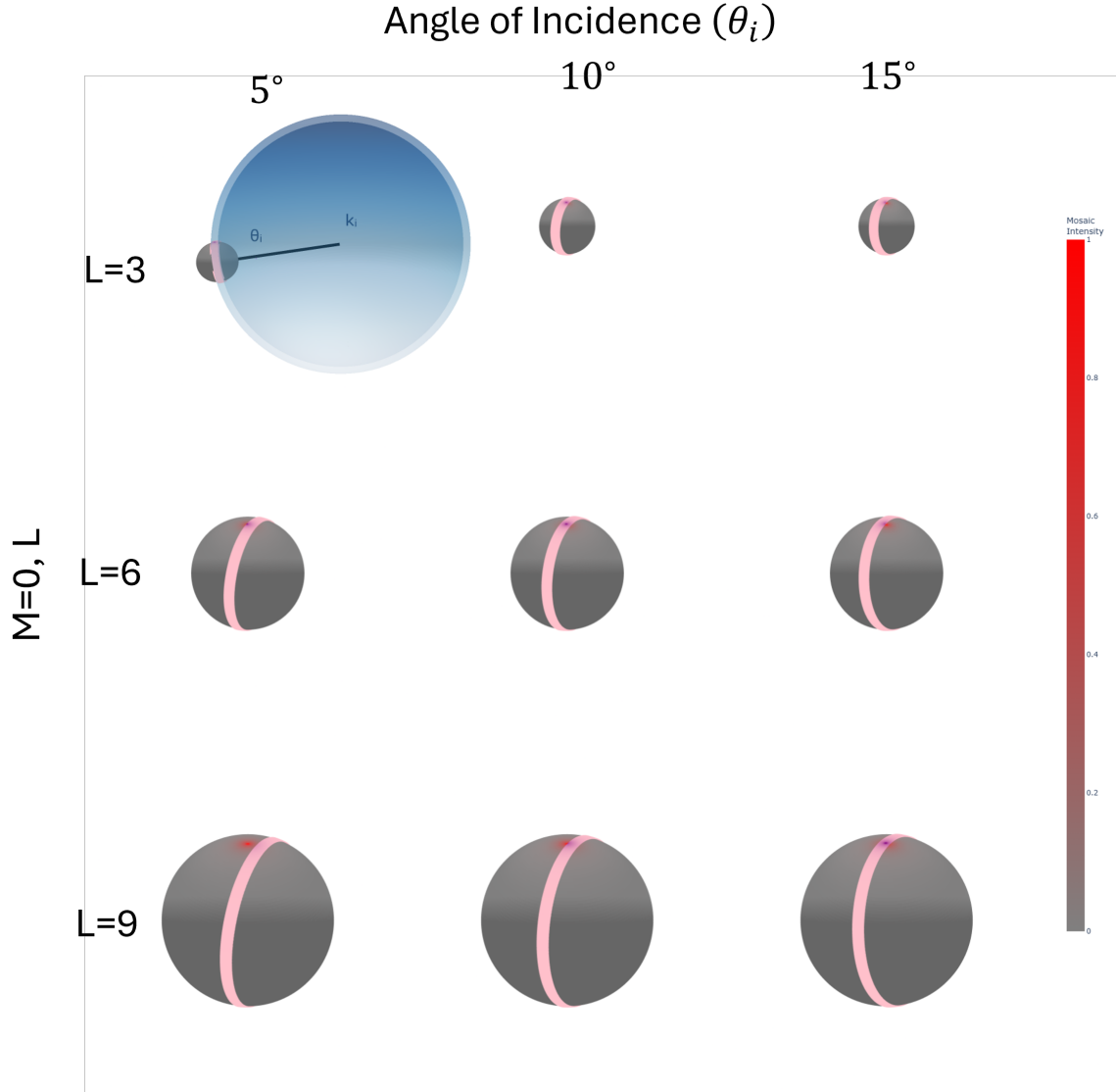
Figure 6: Comparison of small and large Bragg spheres (grey) shows the Ewald-sphere (blue and only shown in the L=3 , 5^\circ case) intersection from wavelength bandwidth and mosaic cap. The same instrumental bandwidth can sample a much larger angular fraction of a low-order Bragg sphere than of a high-order Bragg sphere. The result is that low-order peaks will survive at higher incident angles than higher-order peaks lower.
