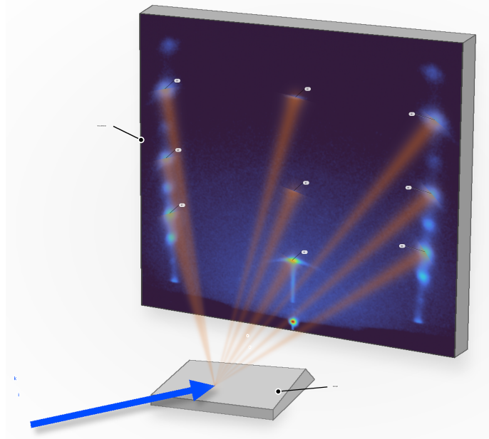
Figure 1: Qualitative area-detector view of a 2D-powder WAXS measurement. The incident beam strikes the film at a shallow angle, and diffracted intensity is recorded directly on the area detector. Labeled bright features indicate representative Bragg peaks, while the extended streaks and arcs illustrate how oriented crystallites, finite mosaic spread, and detector geometry distribute reciprocal-space intensity across the detector image.
