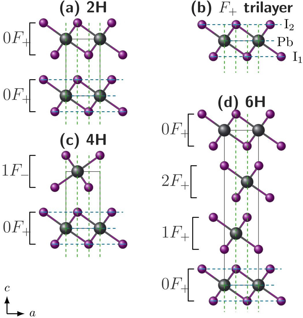
Figure 11: Projected I-Pb-I trilayers for the deterministic \text{PbI}_2 parent cycles used in the transition model. (a) 2H repeats 0F_+ under a = 1 . (b) An isolated F_+ trilayer shows the Pb and I atomic planes used to define the local orientation. (c) 4H alternates 0F_+ and 1F_- under d_+ = 1 . (d) 6H advances 0F_+ \rightarrow 1F_+ \rightarrow 2F_+ \rightarrow 0F_+ under b_+ = 1 . The c axis points upward, so each stack is read from bottom to top. In a state label rF_\sigma , r \in \{0, 1, 2\} is the basal registry and \sigma \in \{+, -\} is the trilayer orientation. Violet and gray spheres denote I and Pb, green vertical guides mark lateral registry, blue horizontal guides mark atomic planes, and brackets group each I-Pb-I trilayer. Nominal ionic signs are shown on the reference F_+ trilayer.
