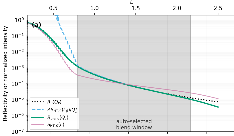
Figure 8: Optical-to-structural handoff used for the near-critical specular-family calculation. (a) Pure Parratt reflectivity gives the low- Q_z optical response, including refraction, evanescence, and multiple reflection at the film interfaces. The high- Q_z branch is the normalized finite-stack structure term scaled to the optical branch in an overlap region. The final curve is a smooth log-intensity blend between these limits, plotted versus Q_z/Q_c with the corresponding crystallographic L coordinate on the top axis.
