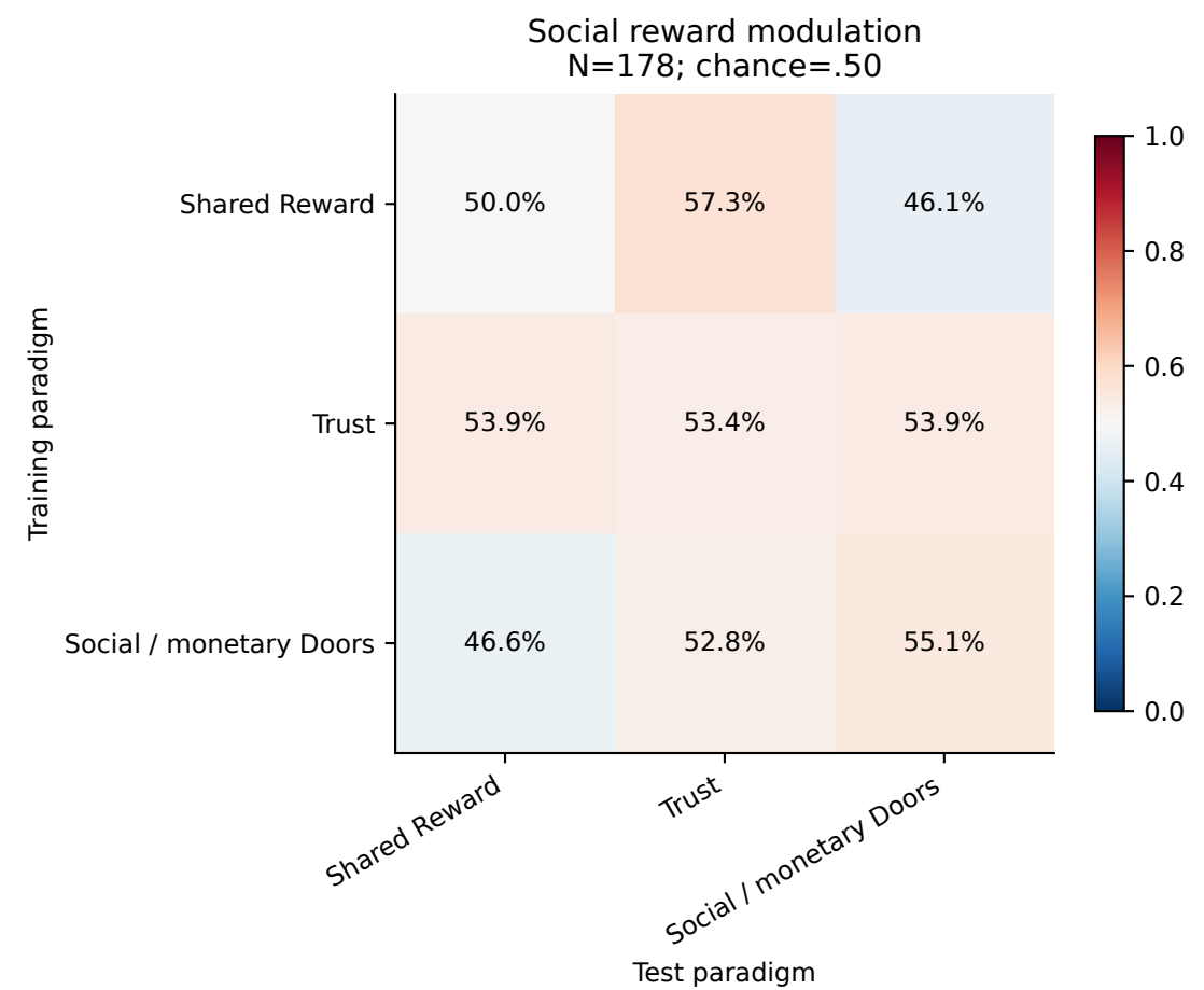
Figure 2. Social context versus social reward modulation
