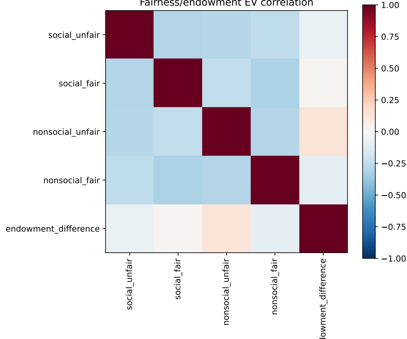
Fairness/endowment EV correlation
