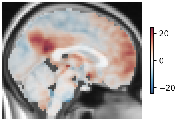
Friend-stranger context positive; x \approx 0 mm
