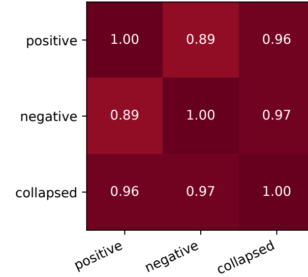
Haufe spatial correlation
