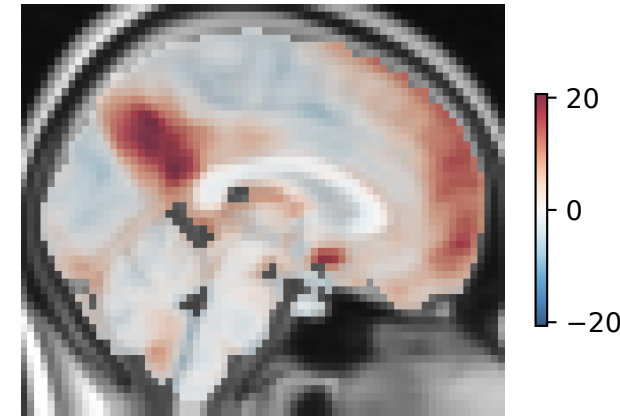
Social context collapsed; x \approx 0 mm
