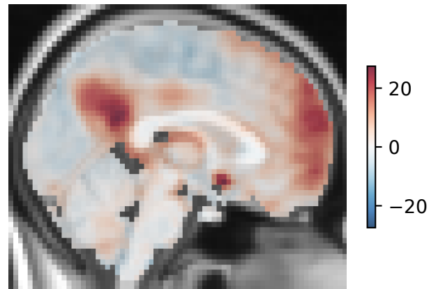
Friend-stranger context negative; x \approx 0 mm
