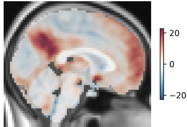
Social context negative; x \approx 0 mm
