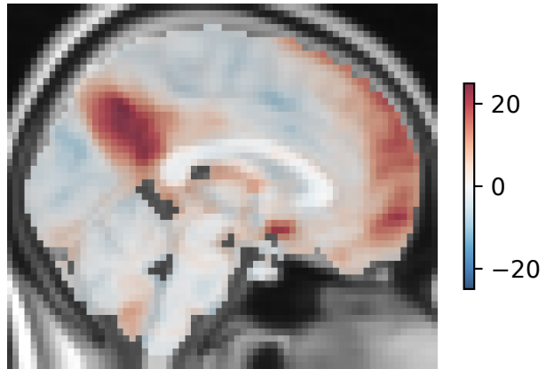
Social context positive; x \approx 0 mm
