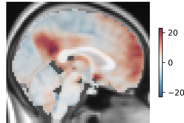
Friend-stranger context collapsed; x \approx 0 mm
