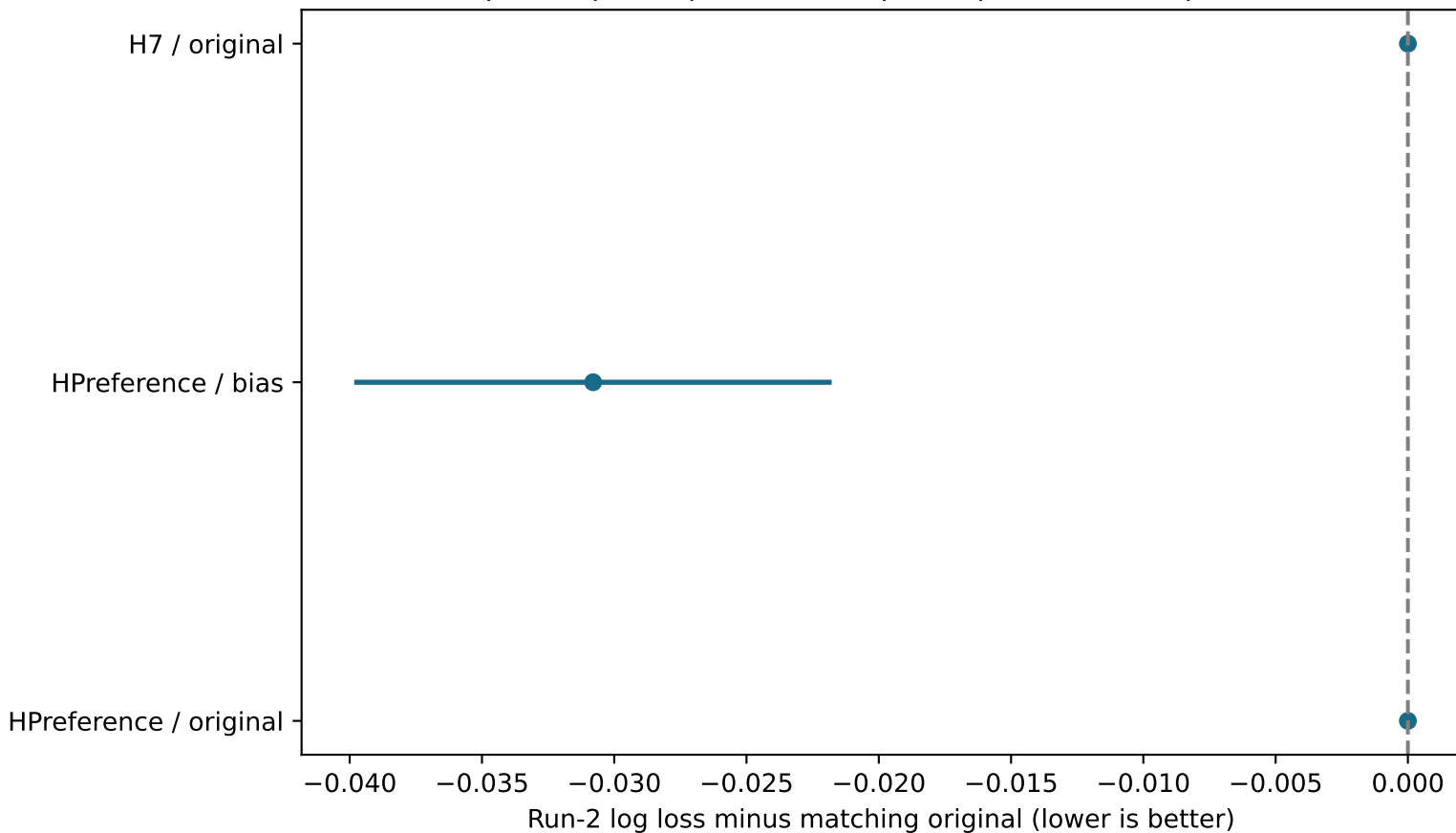
Exploratory amount comparison: 3 accepted models of 6 304 paired participants · 95% participant bootstrap intervals
