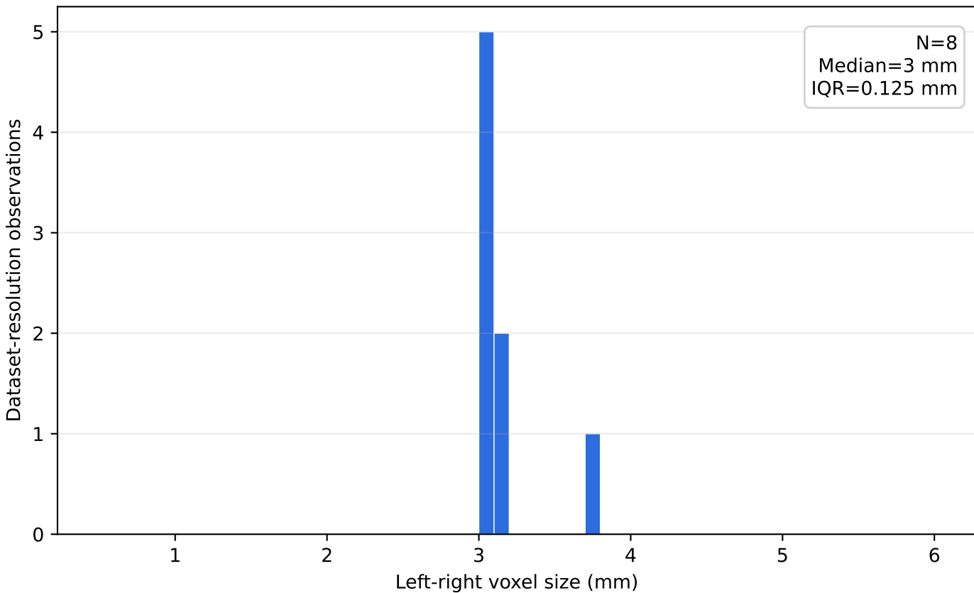
OpenNeuro BOLD voxel size: LR axis
