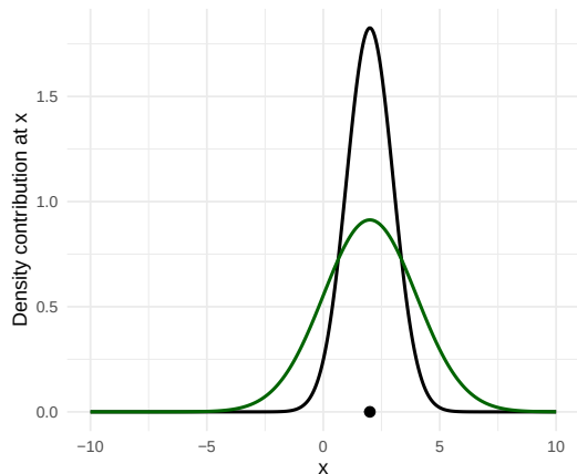
Kernel centered at one data point, different band
