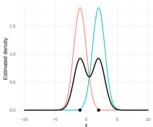
Kernel Density Estimator (KDE) for two data points
