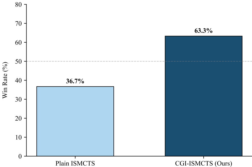
Ablation Study: Effect of Constraint Network
