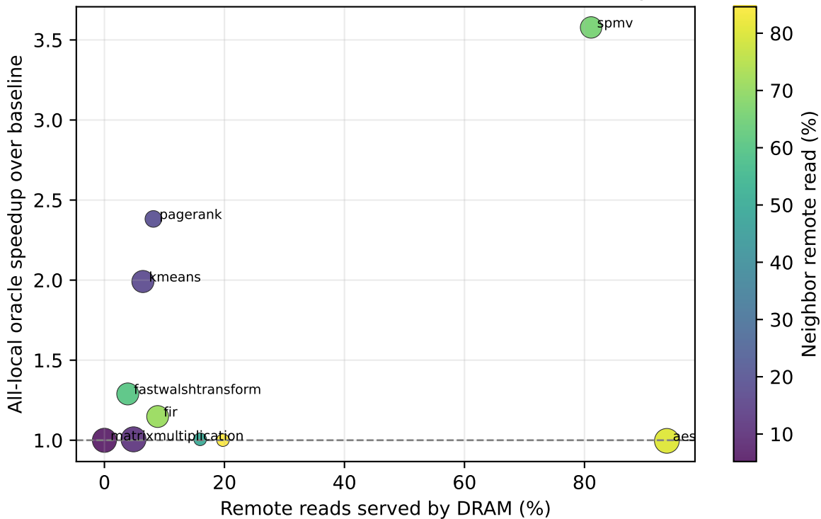
Remote DRAM service vs bottleneck sensitivity
