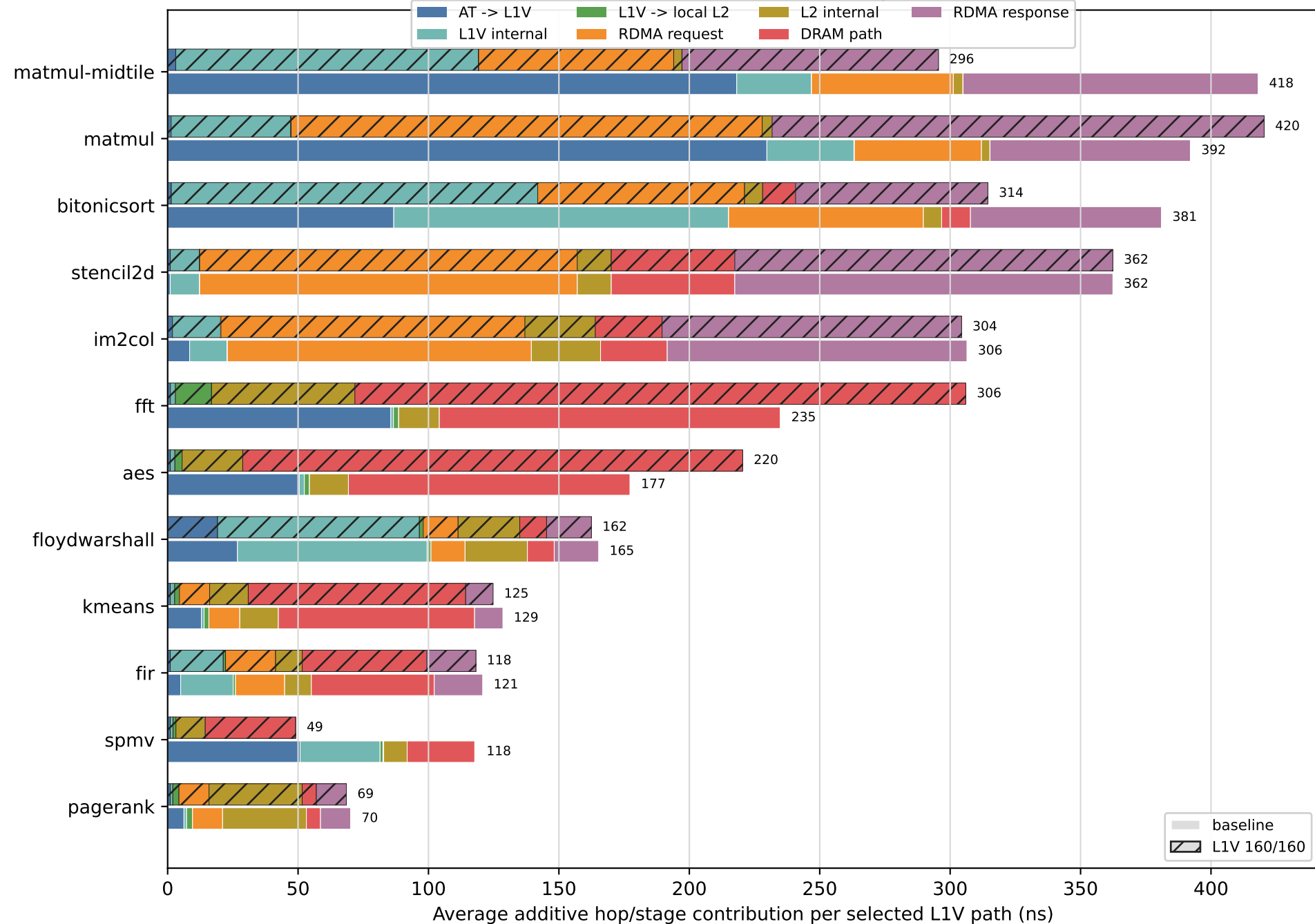
Traditional workloads: baseline vs. L1V 160-MSHR/160-transaction window
