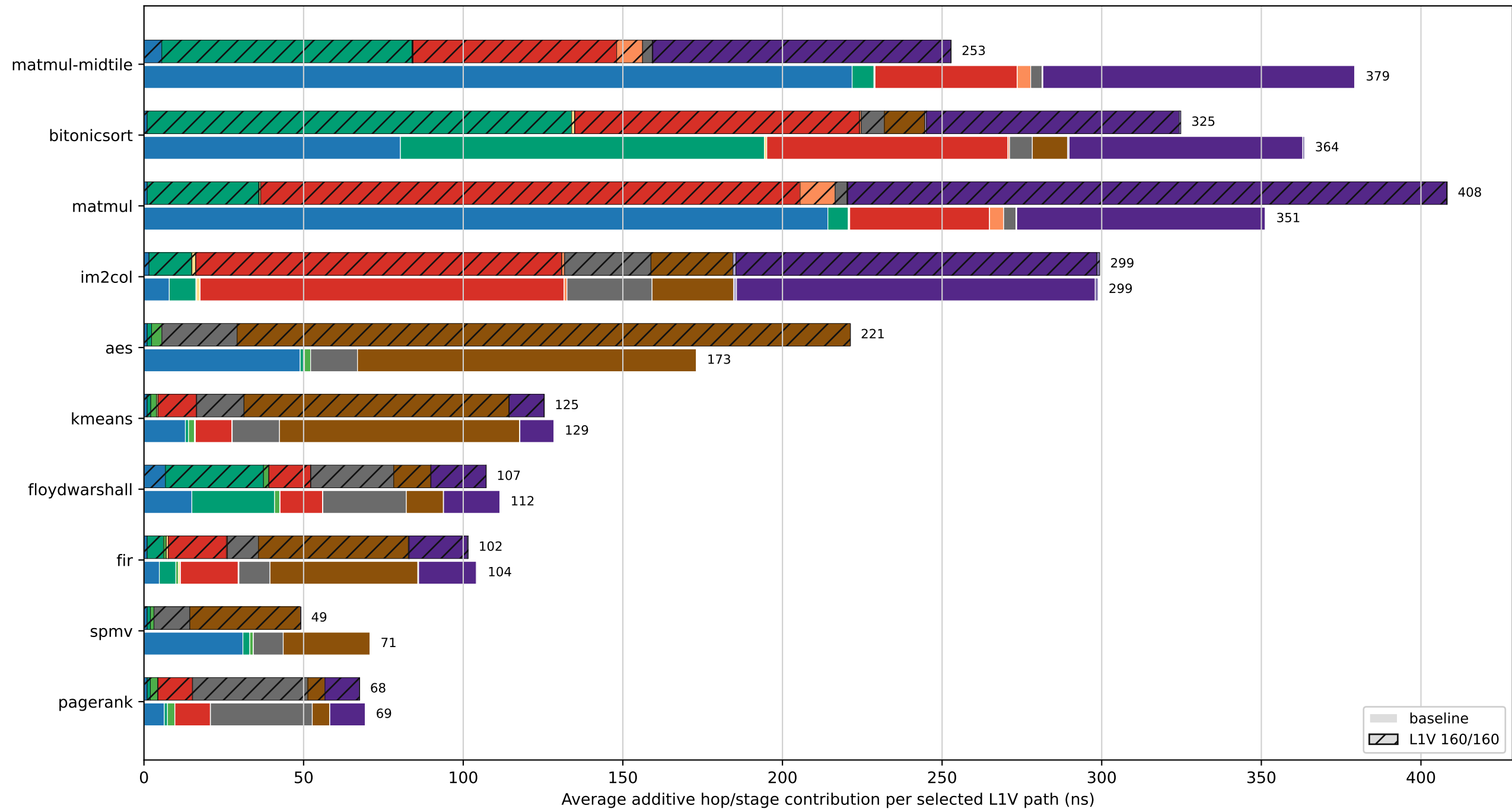
Traditional workloads: baseline vs. L1V 160/160 with expanded RDMA breakdown
