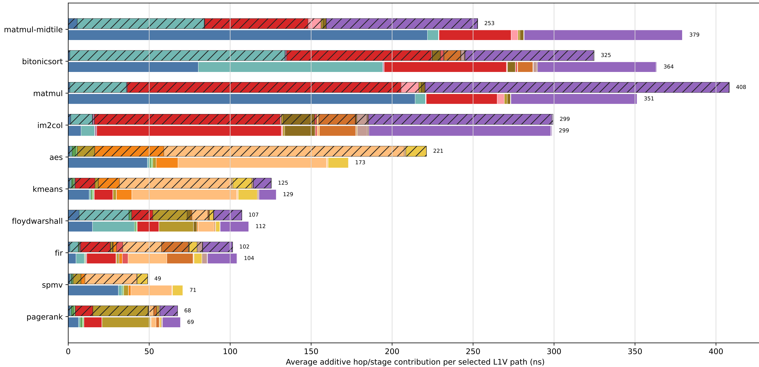
Traditional workloads: baseline vs. L1V 160-MSHR/160-transaction window
