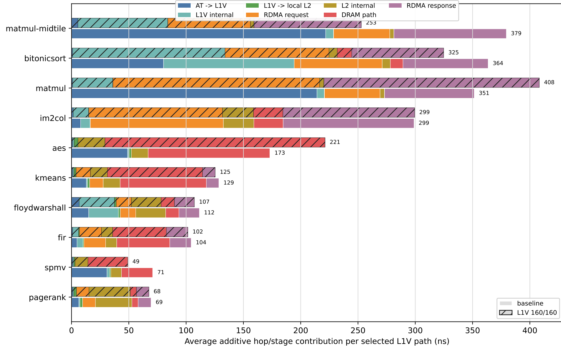
Traditional workloads: baseline vs. L1V 160-MSHR/160-transaction window
