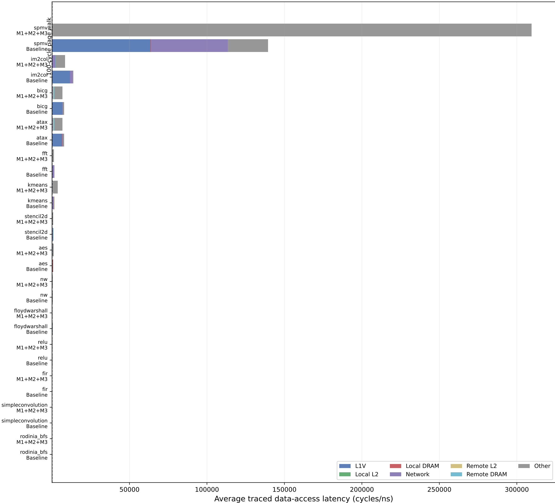
Data-access critical-path breakdown, post-warmup traces
