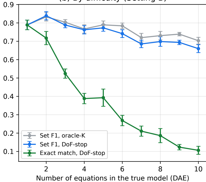
(b) By difficulty (Setting B)
