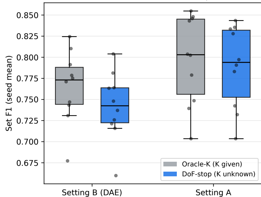
(a) Oracle-K vs. DoF-stop
