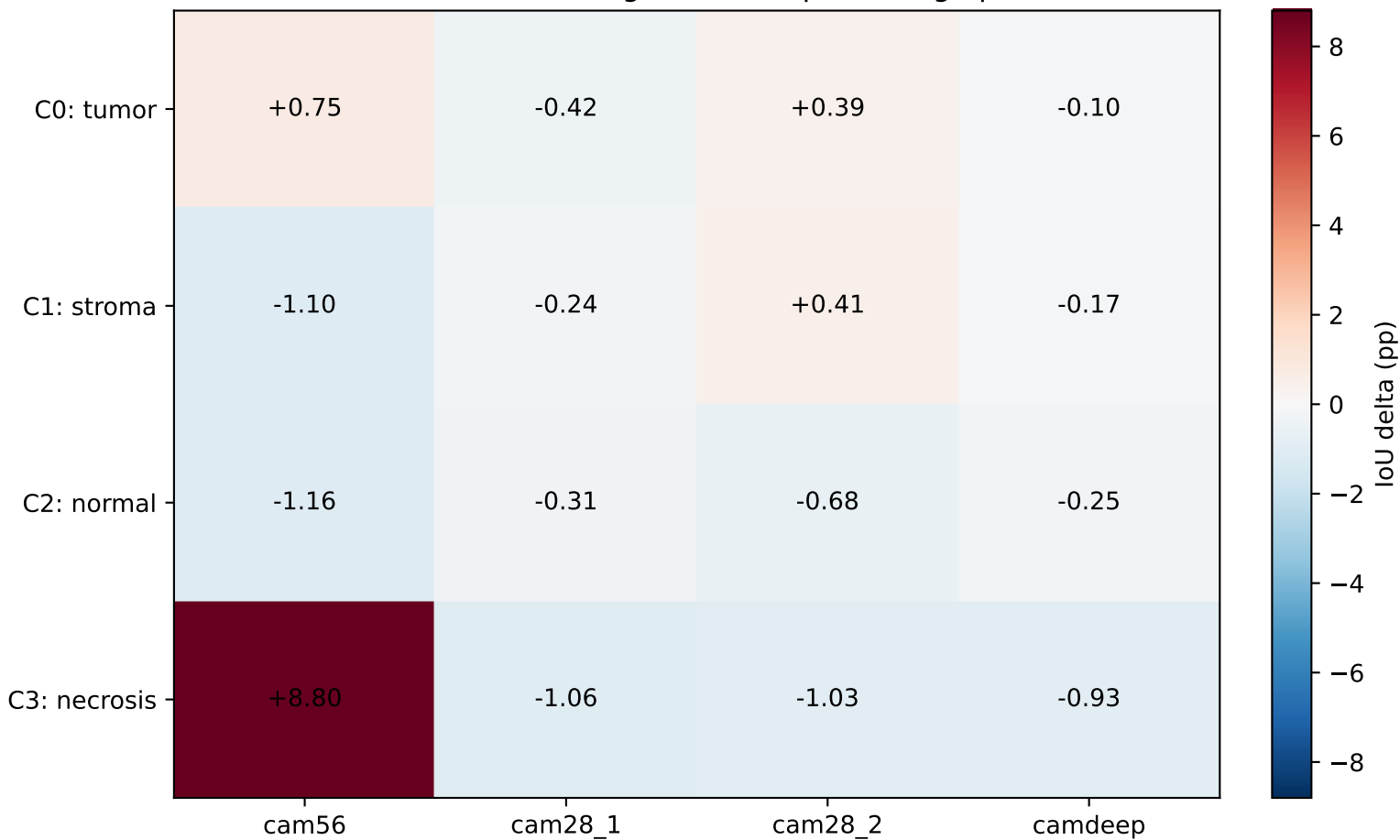
FA-MPR minus A0 stagewise IoU (percentage points)
