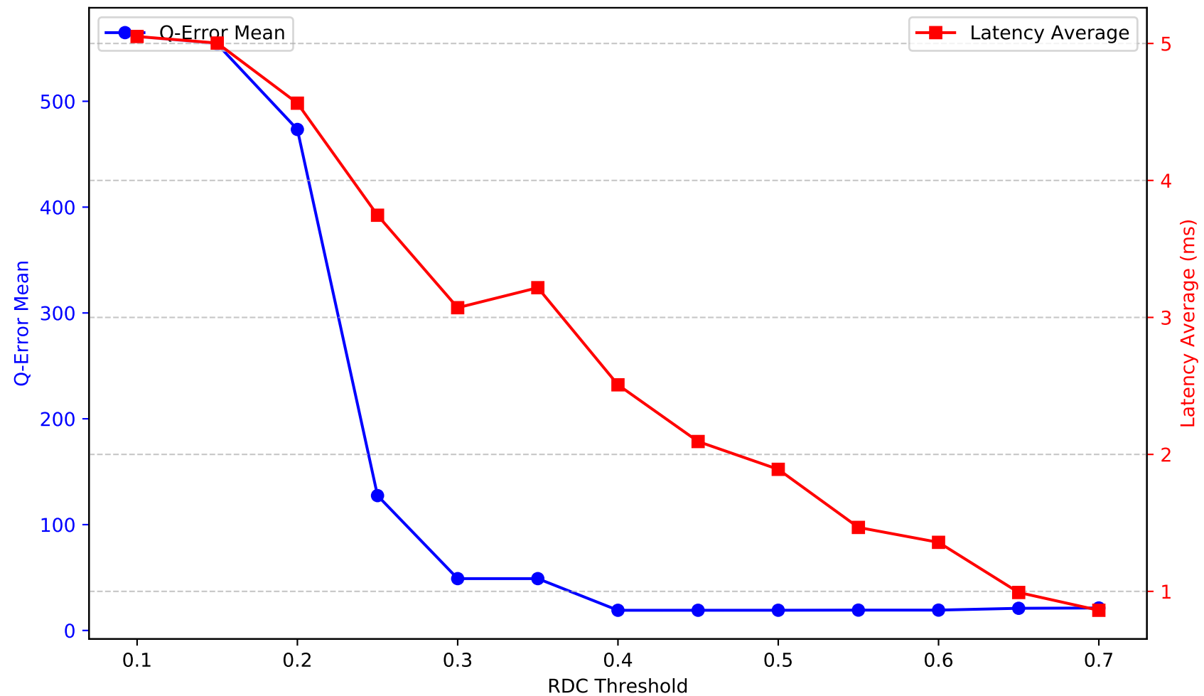
Metrics by RDC Threshold - testpad_pcb_xyrgb_v2
