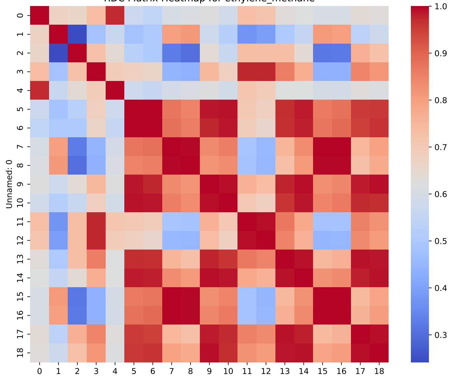
RDC Matrix Heatmap for ethylene_methane
