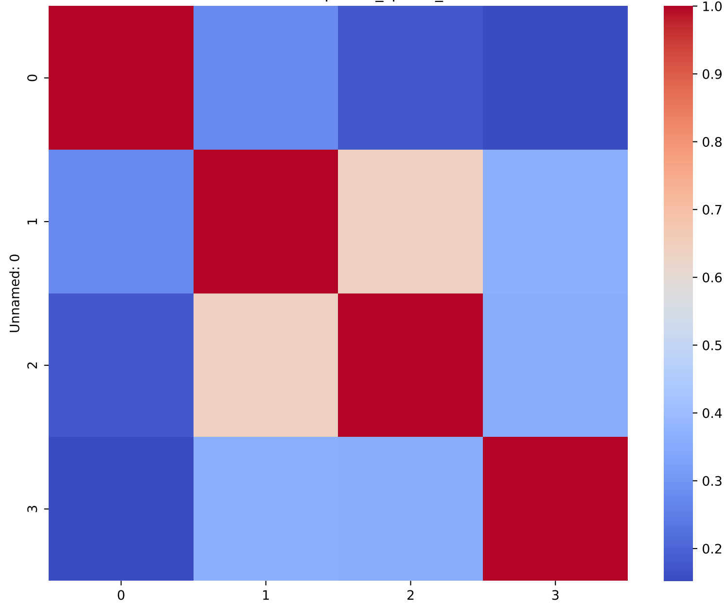
RDC Matrix Heatmap for d_spatial_network
