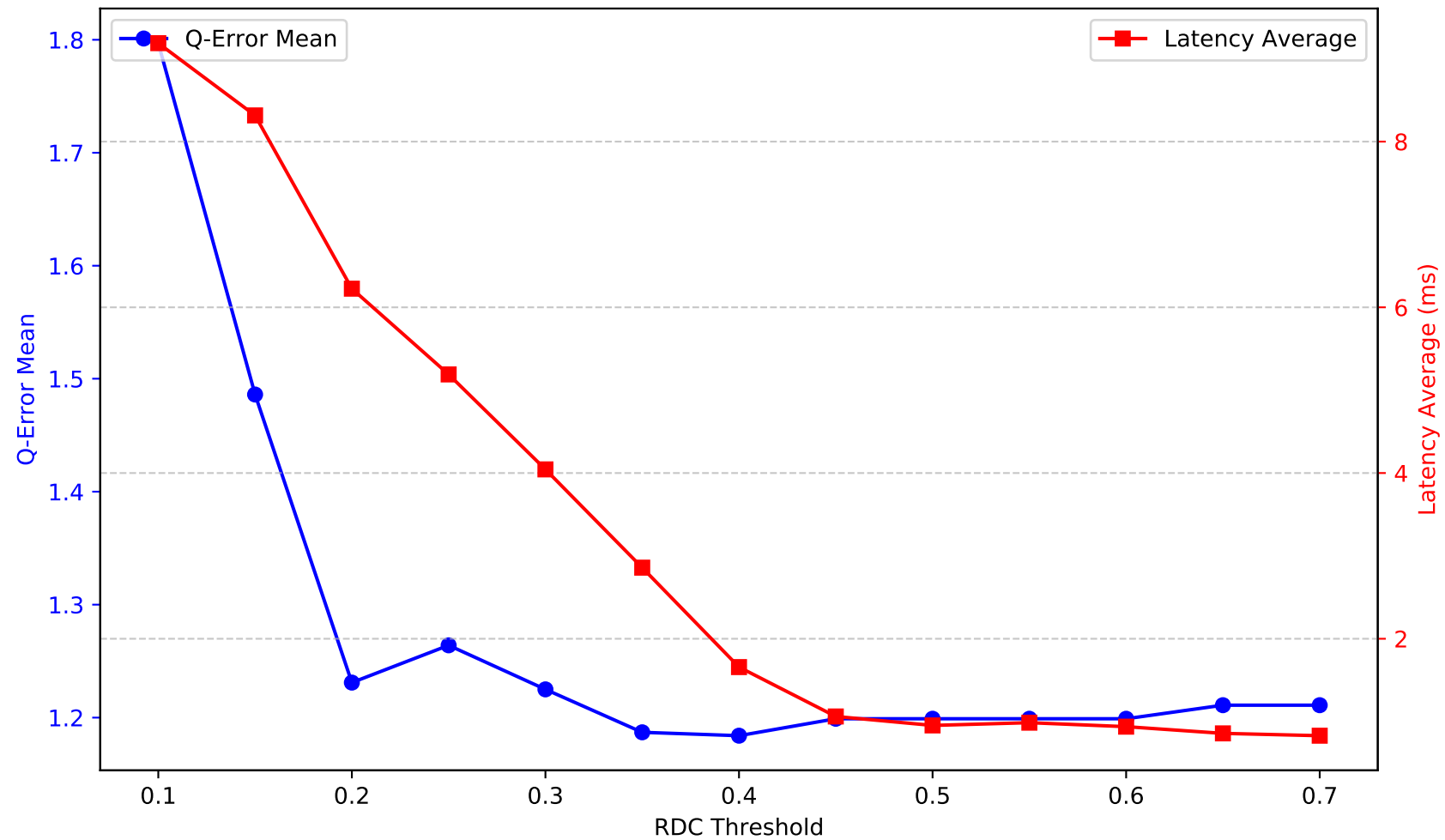
Metrics by RDC Threshold - nhanes_age_prediction
