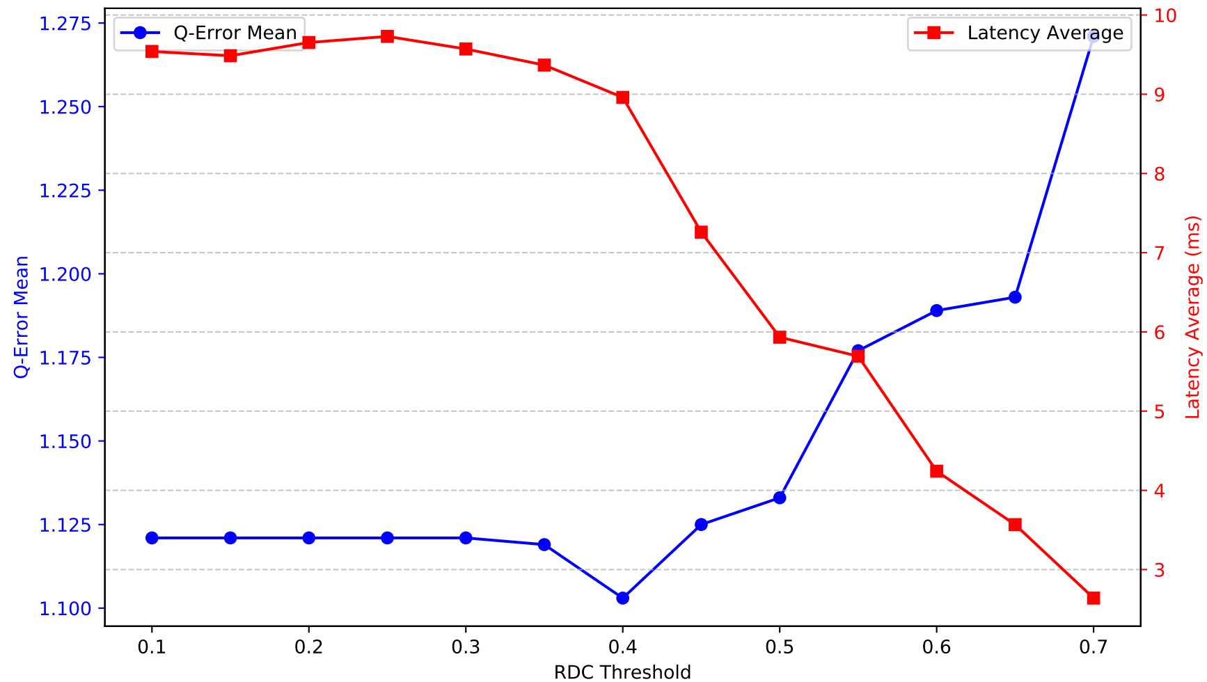
Metrics by RDC Threshold - gt_2011
