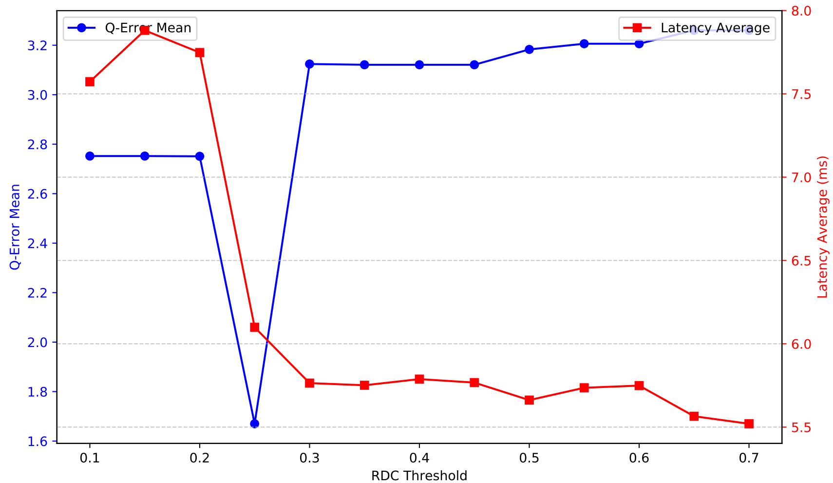
Metrics by RDC Threshold - pricerunner_aggregate
