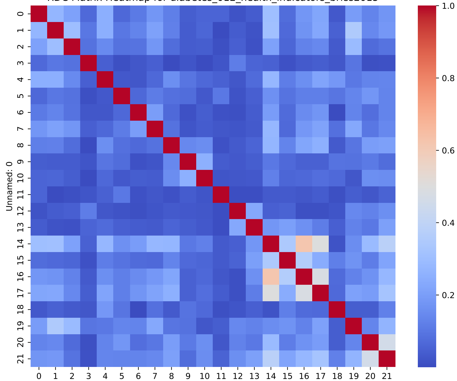
RDC Matrix Heatmap for diabetes_012_health_indicators_brfss2015
