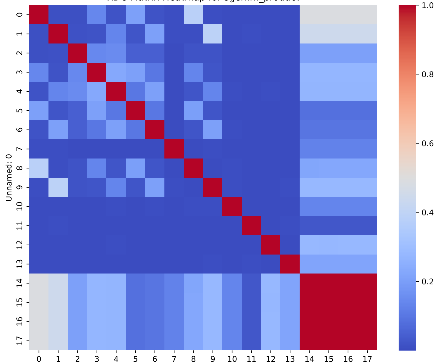
RDC Matrix Heatmap for sgemm_product
