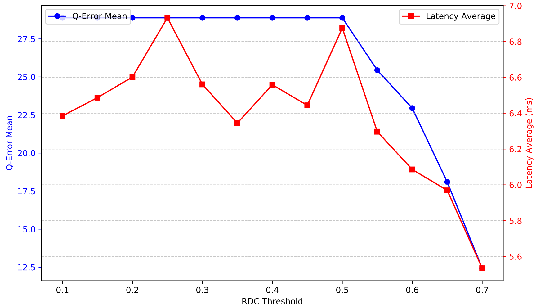
Metrics by RDC Threshold - database_gas
