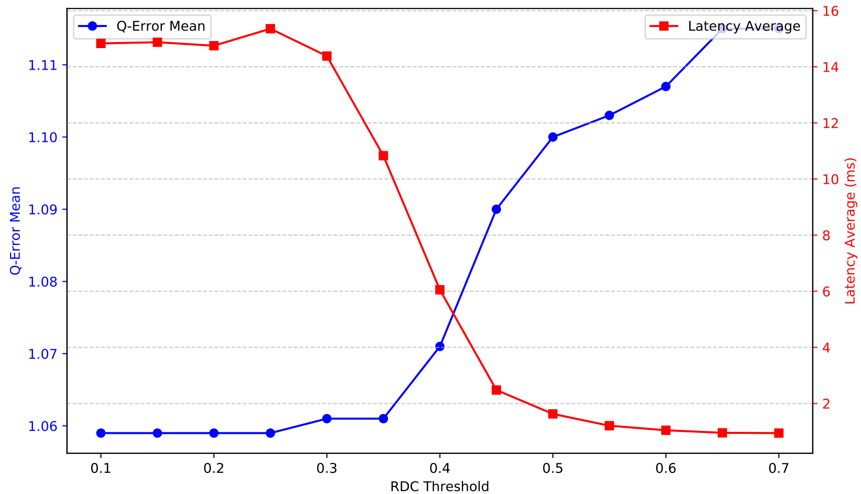
Metrics by RDC Threshold - yearpredictionmsd
