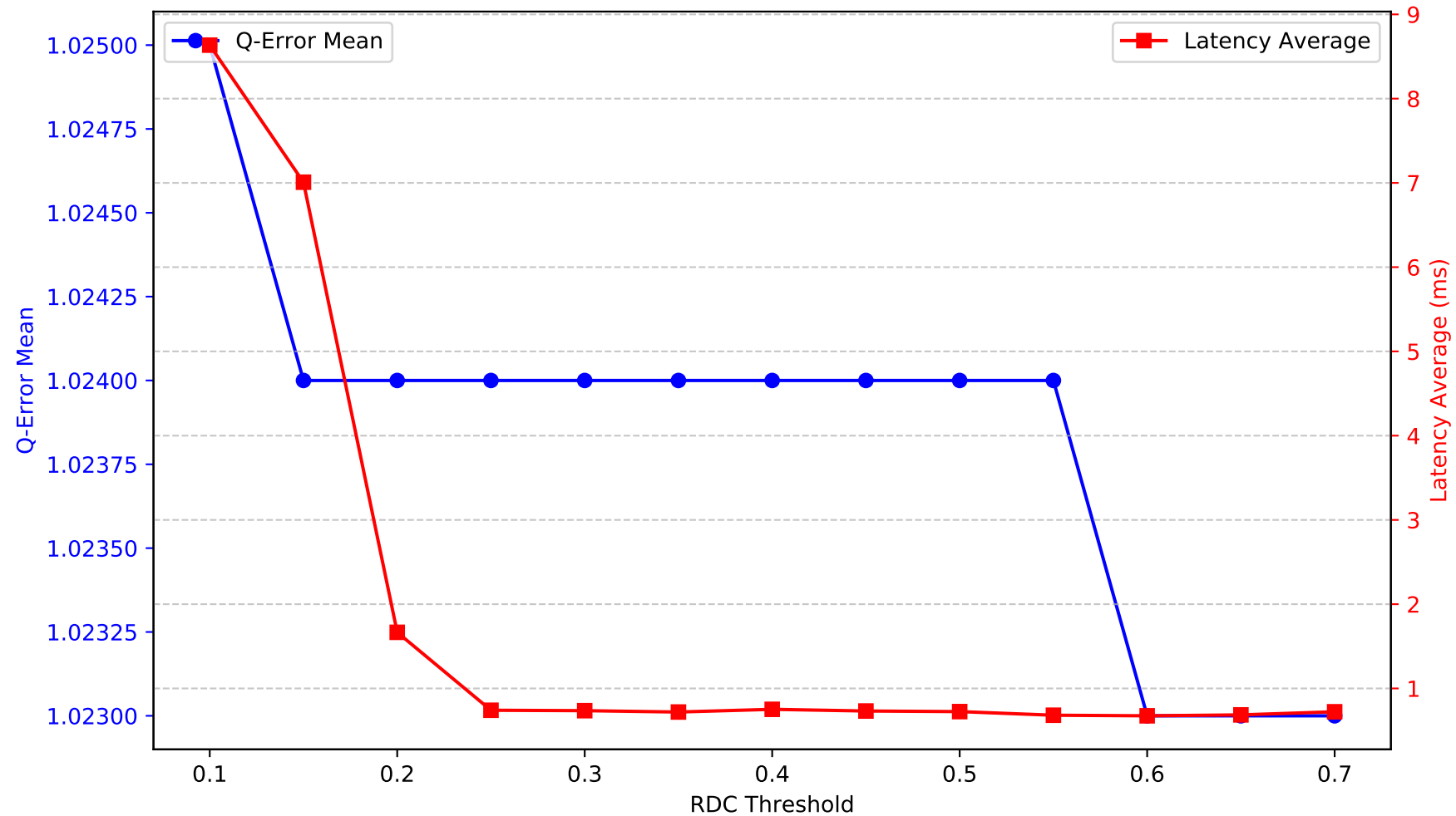
Metrics by RDC Threshold - raw1
