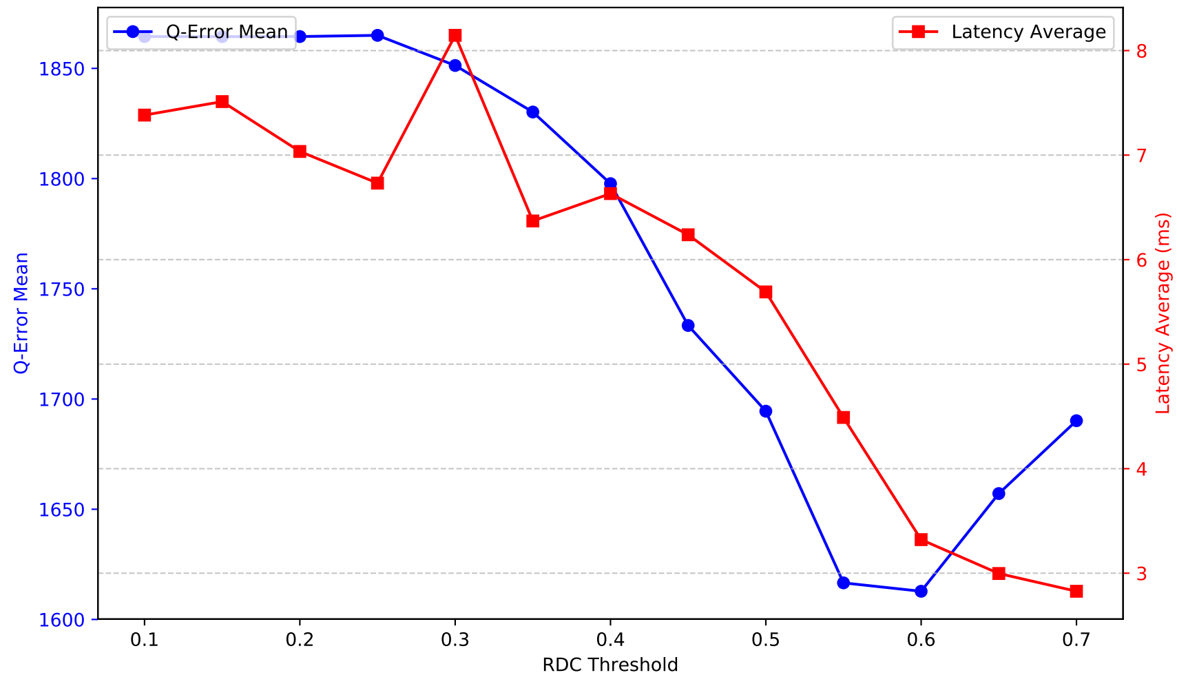
Metrics by RDC Threshold - metrop3
