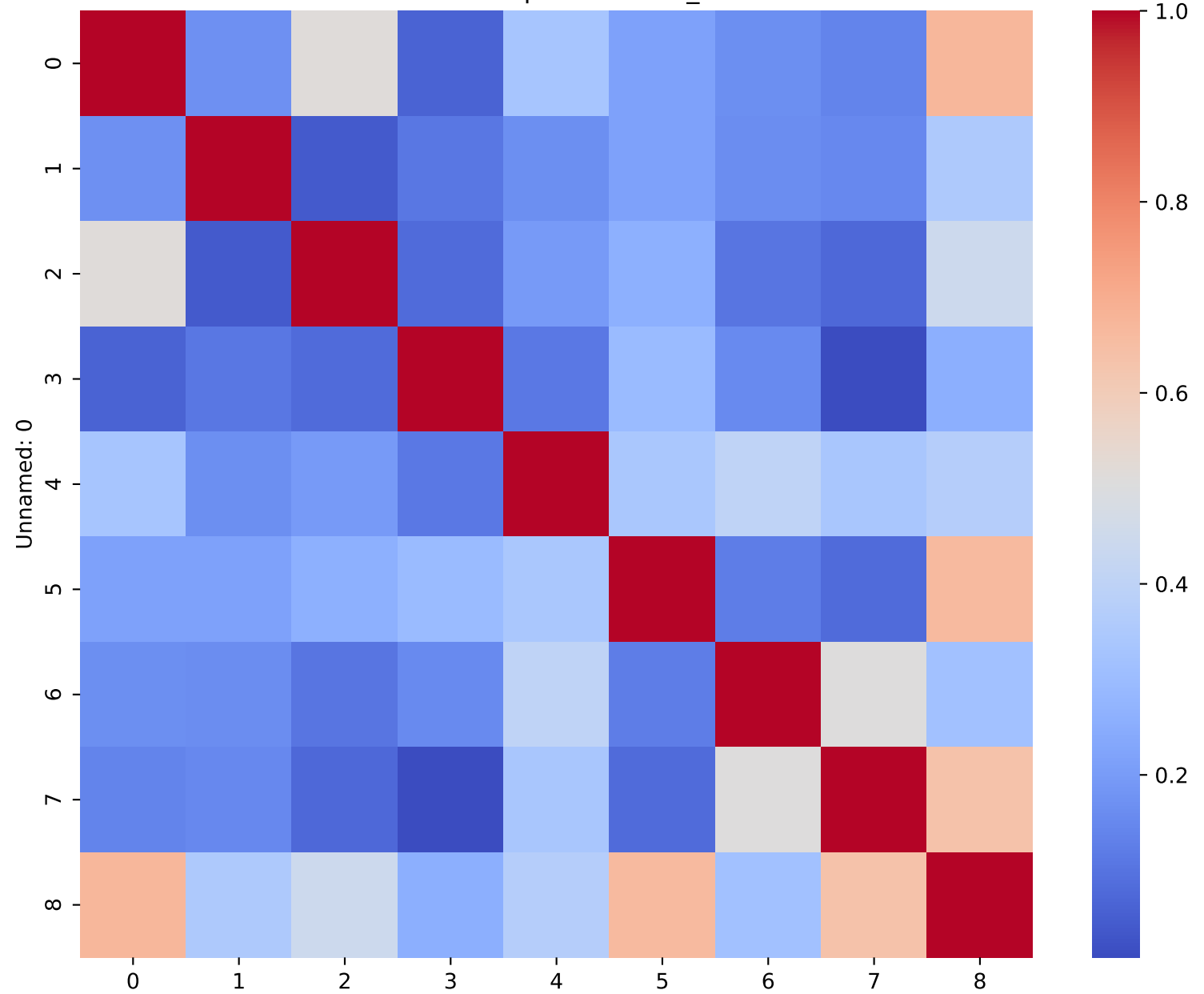
RDC Matrix Heatmap for auction_verification
