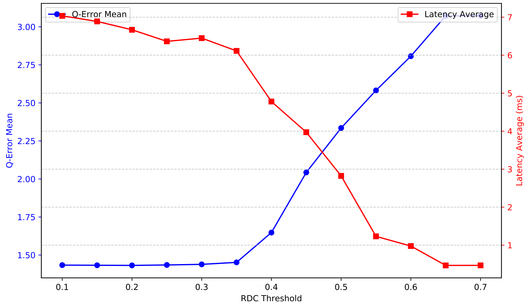
Metrics by RDC Threshold - auction_verification
