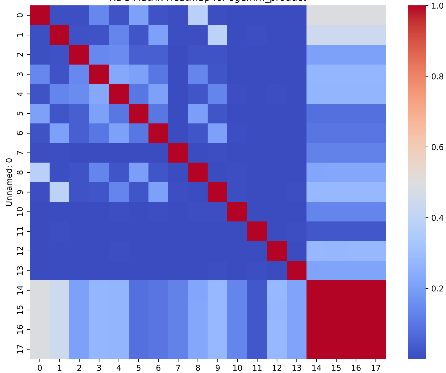
RDC Matrix Heatmap for sgemm_product
