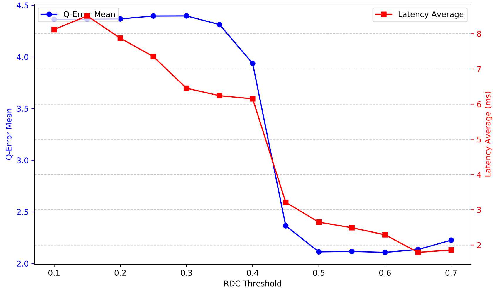
Metrics by RDC Threshold - recipereviews
