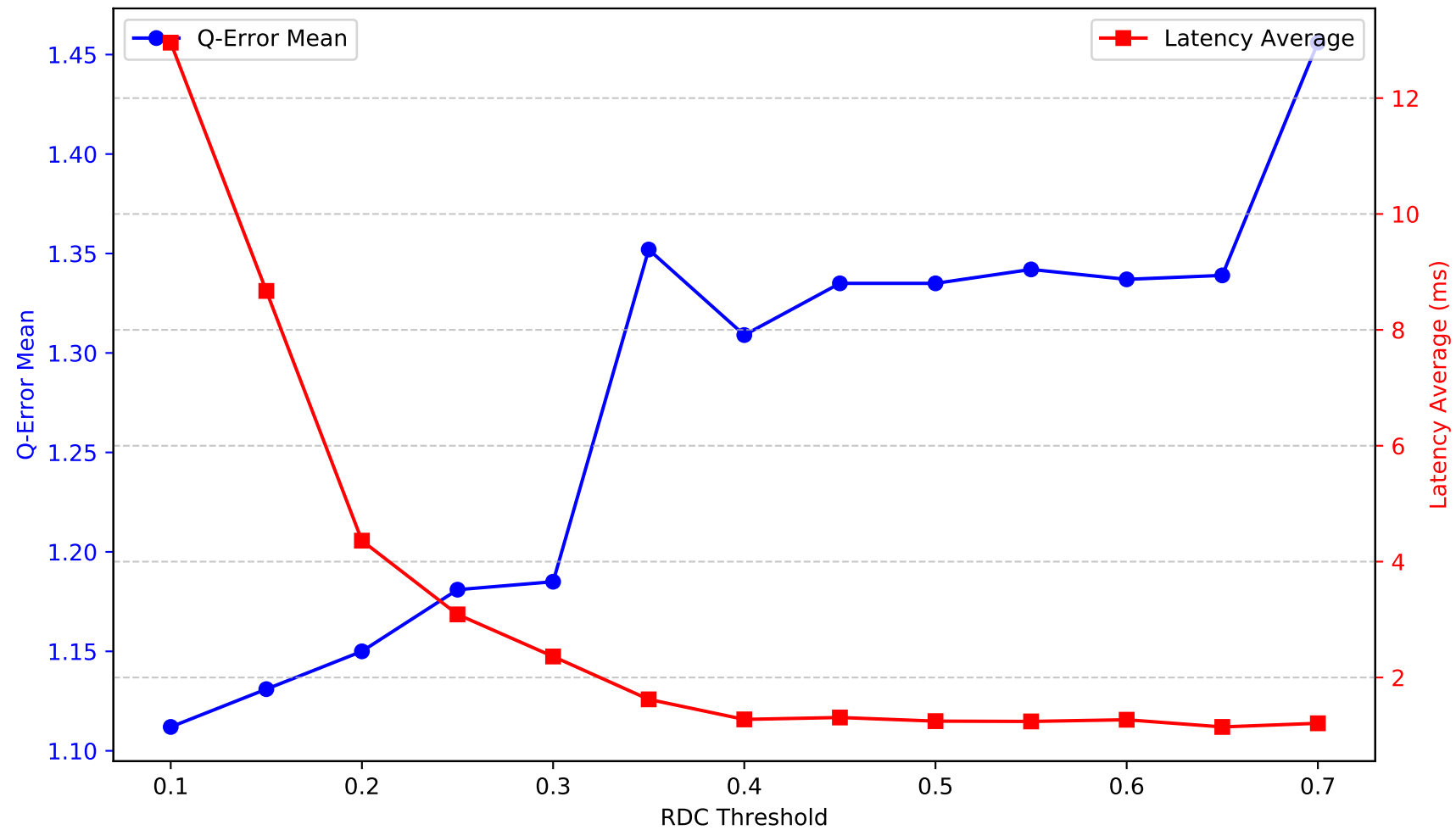
Metrics by RDC Threshold - naticusdroid
