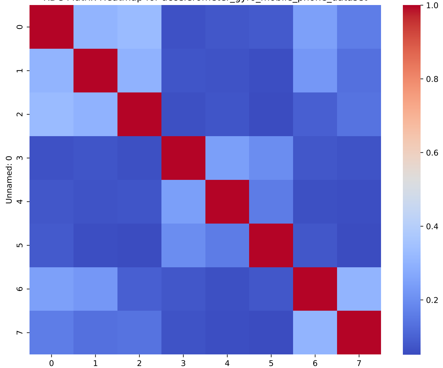
RDC Matrix Heatmap for accelerometer_gyro_mobile_phone_dataset
