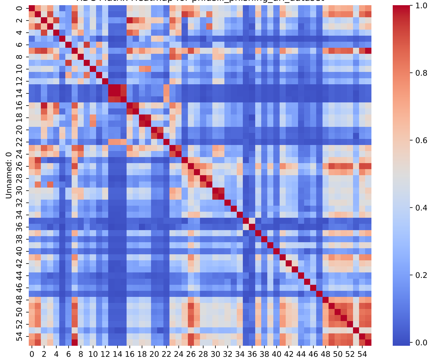
RDC Matrix Heatmap for phiusiil_phishing_url_dataset
