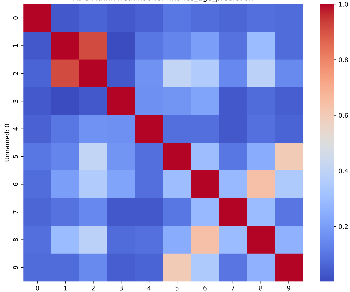
RDC Matrix Heatmap for nhanes_age_prediction
