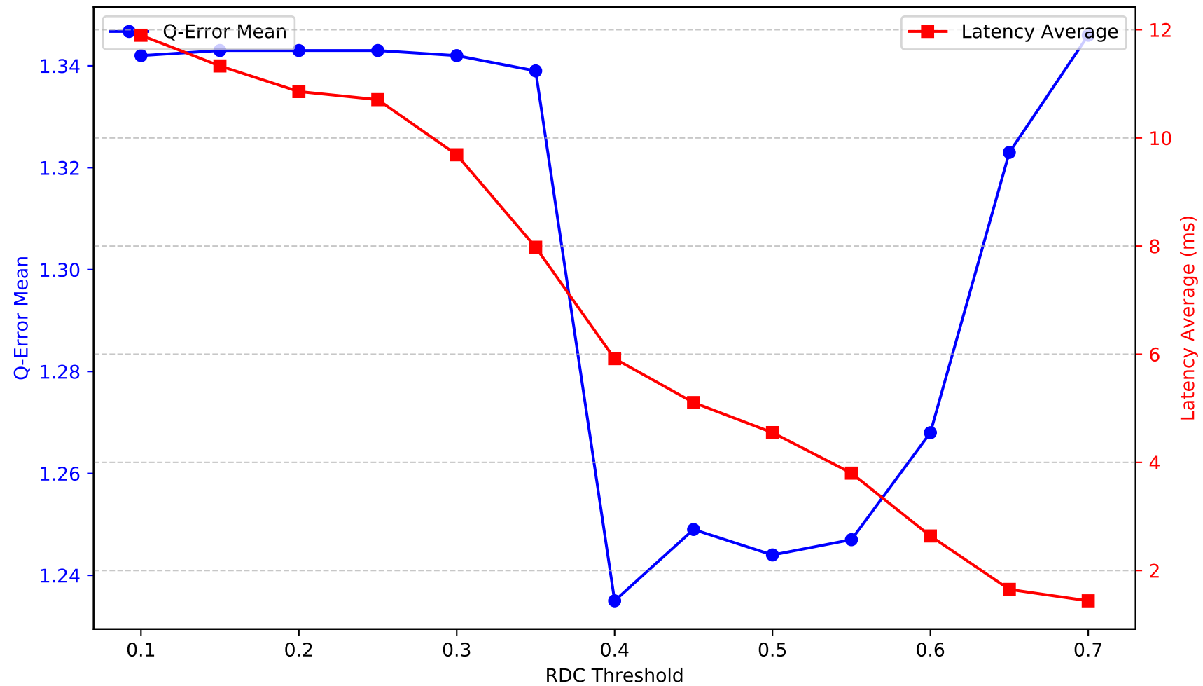
Metrics by RDC Threshold - support2
