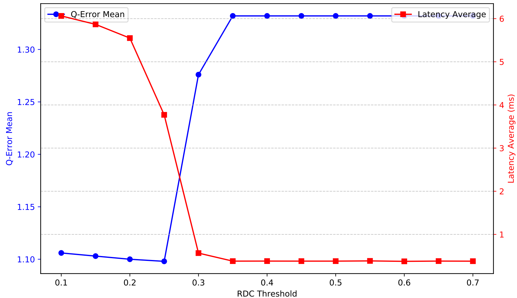
Metrics by RDC Threshold - data1
