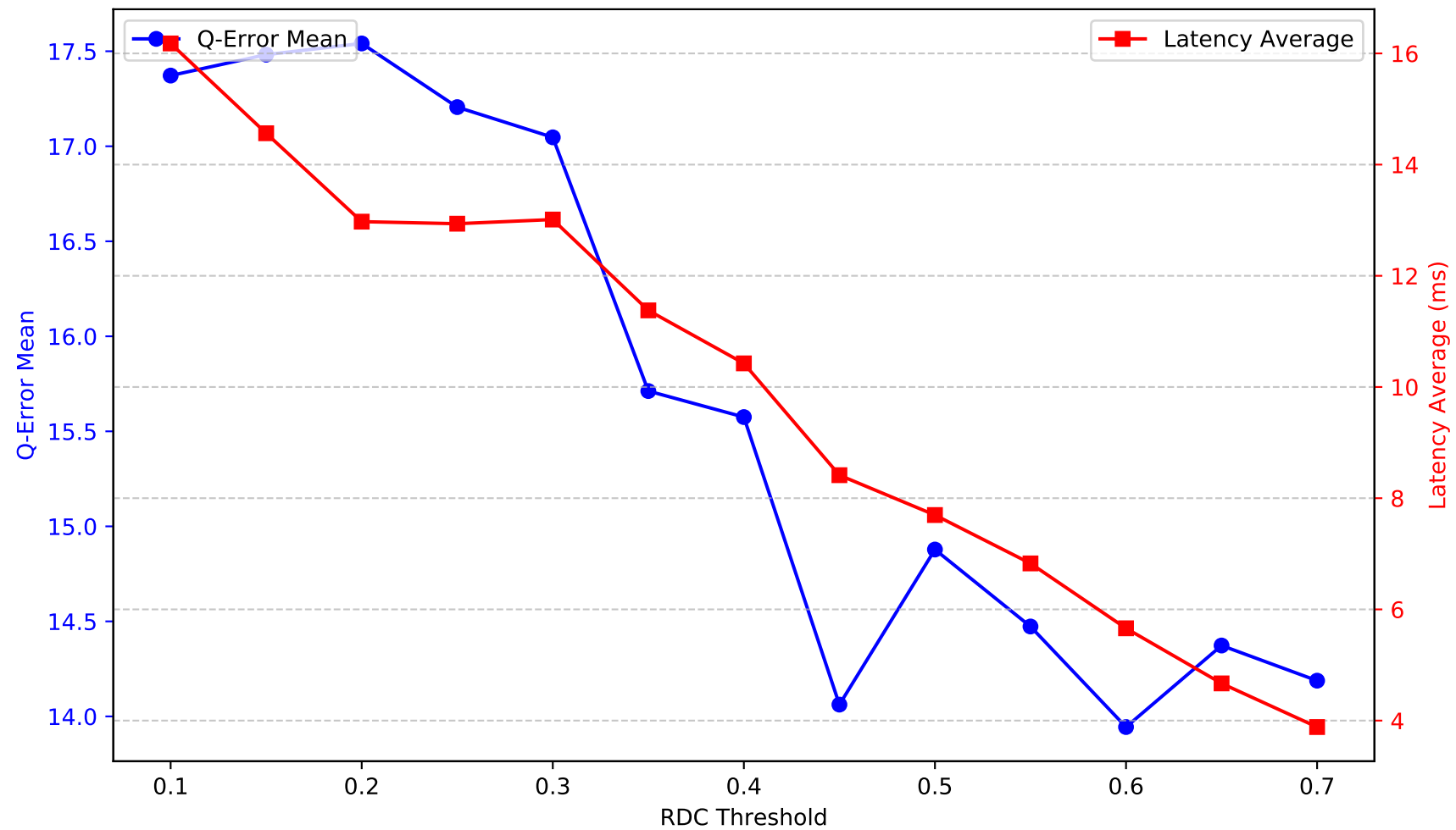
Metrics by RDC Threshold - phiusiil_phishing_url_dataset
