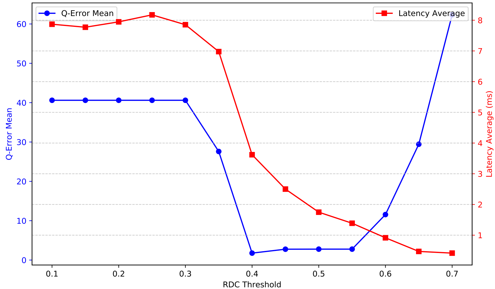
Metrics by RDC Threshold - d_spatial_network
