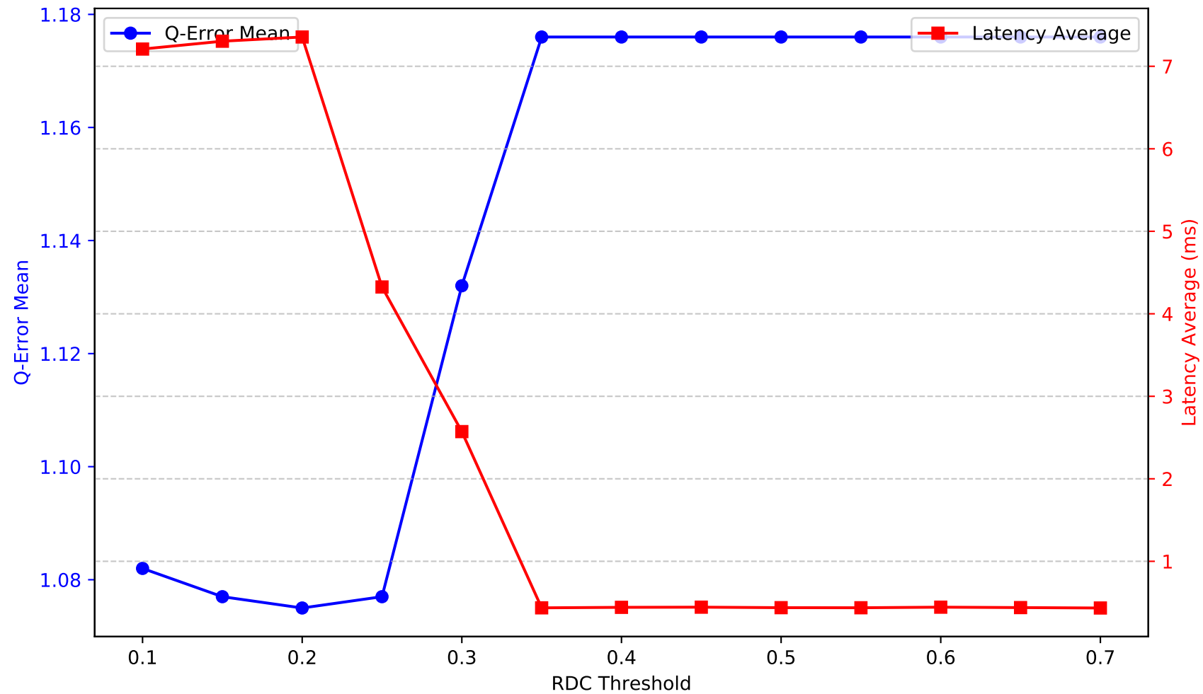
Metrics by RDC Threshold - accelerometer_gyro_mobile_phone_dataset
