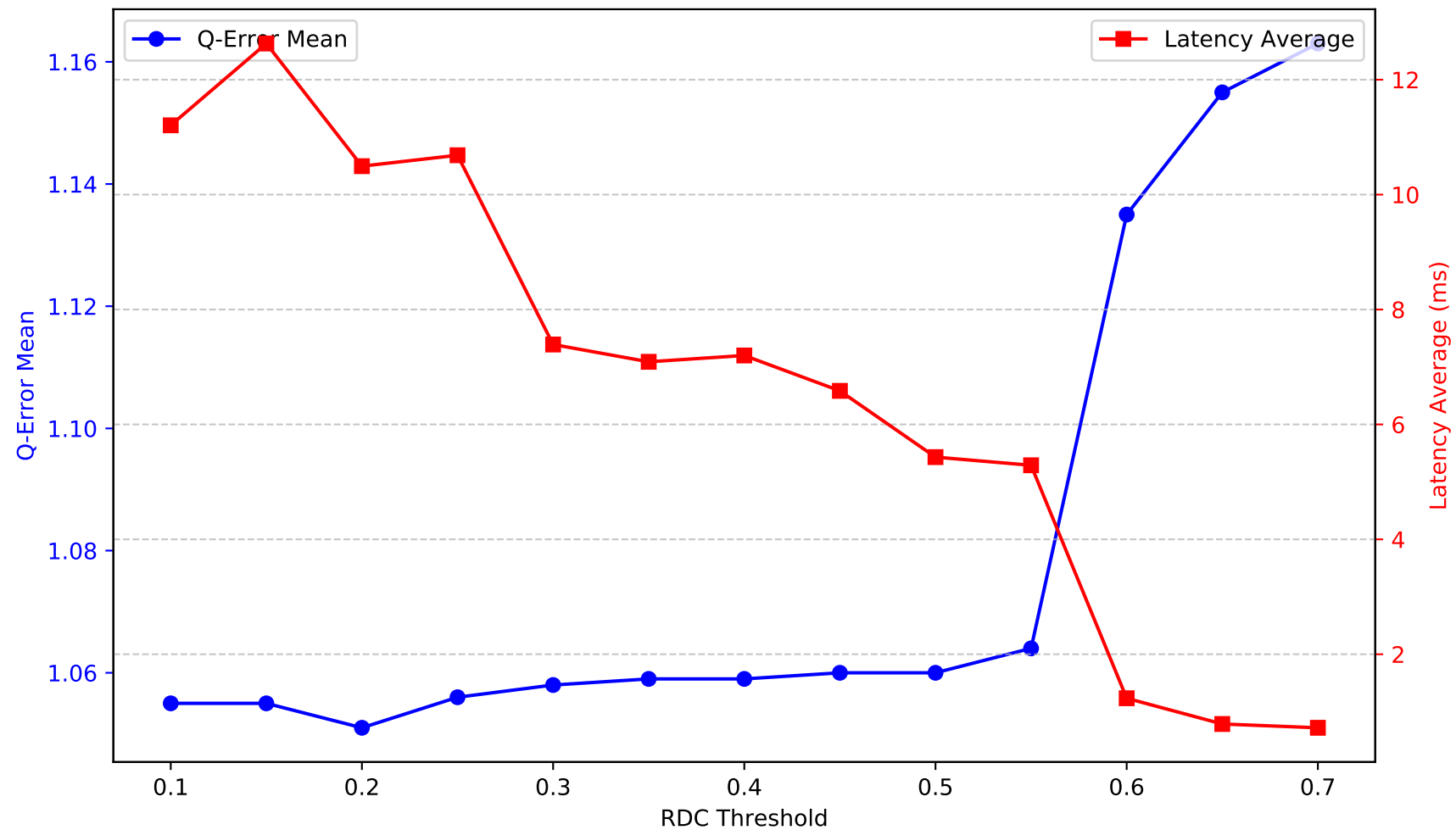
Metrics by RDC Threshold - sydney_data
