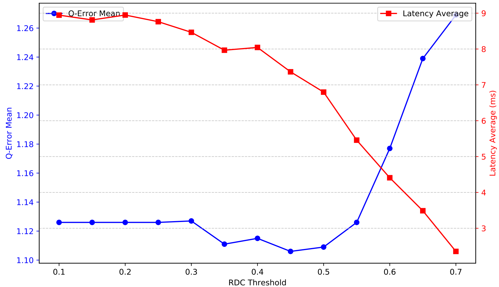
Metrics by RDC Threshold - gt_2015
