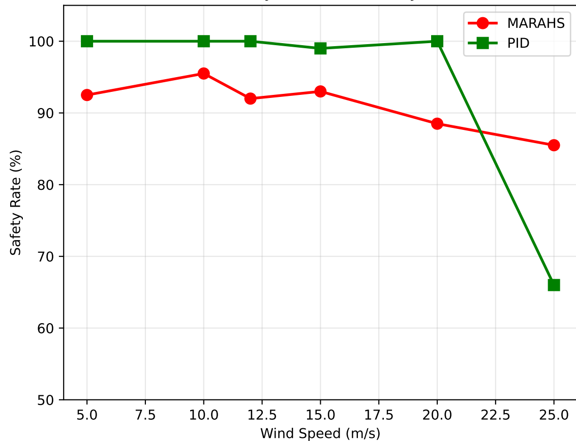
Safety vs Wind Intensity
