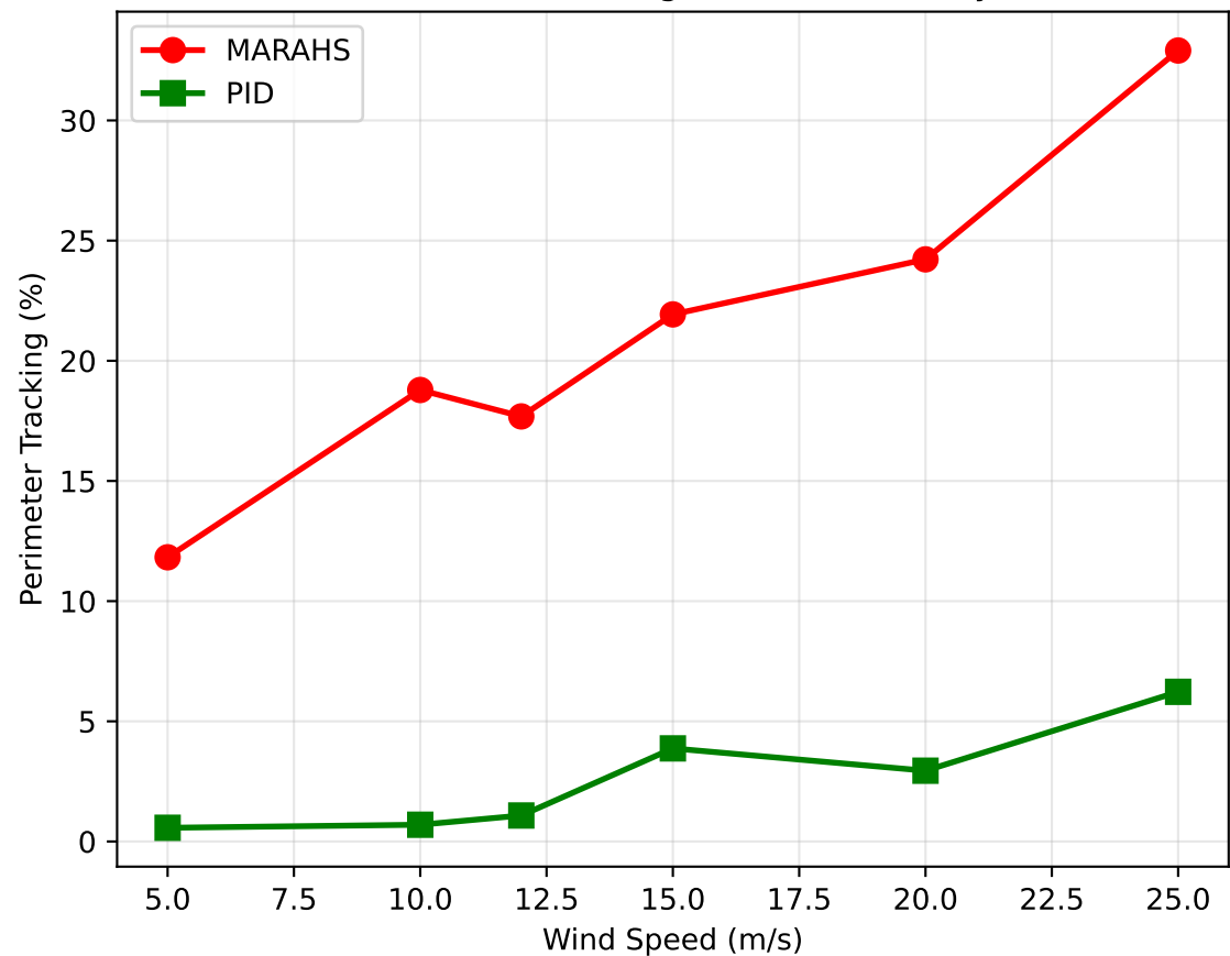
Perimeter Tracking vs Wind Intensity
