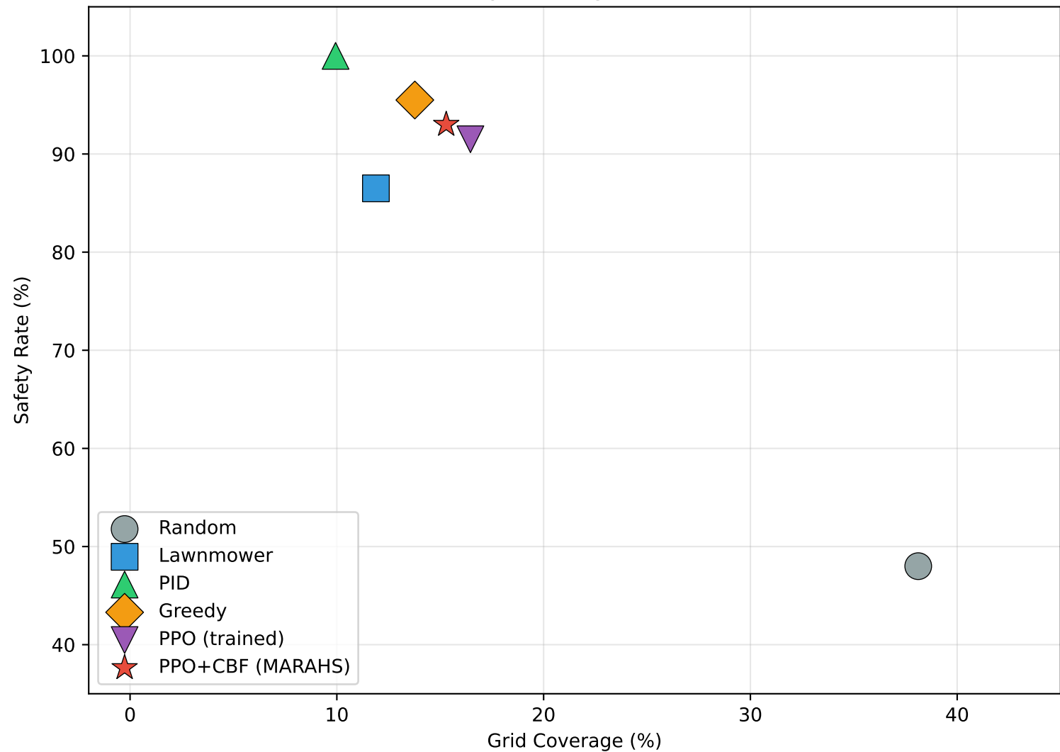
Safety-Coverage Tradeoff
