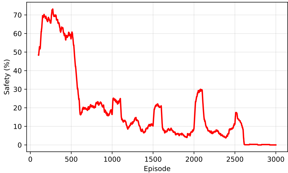
Safety Rate During Training
