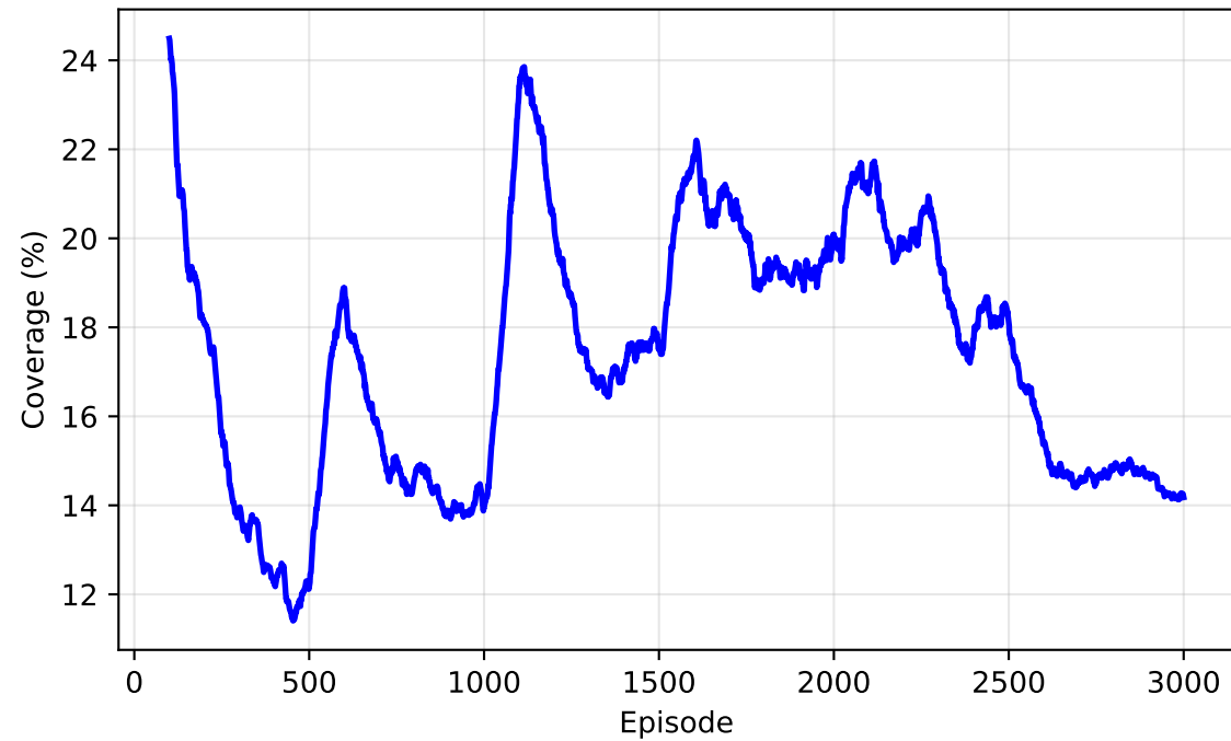
Grid Coverage During Training
