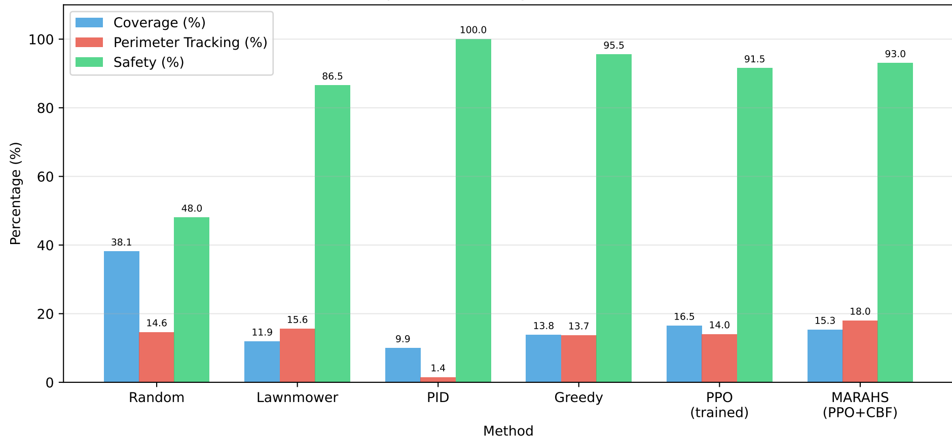
Benchmark Comparison (30×30 grid, 10 drones, wind=12 m/s)
