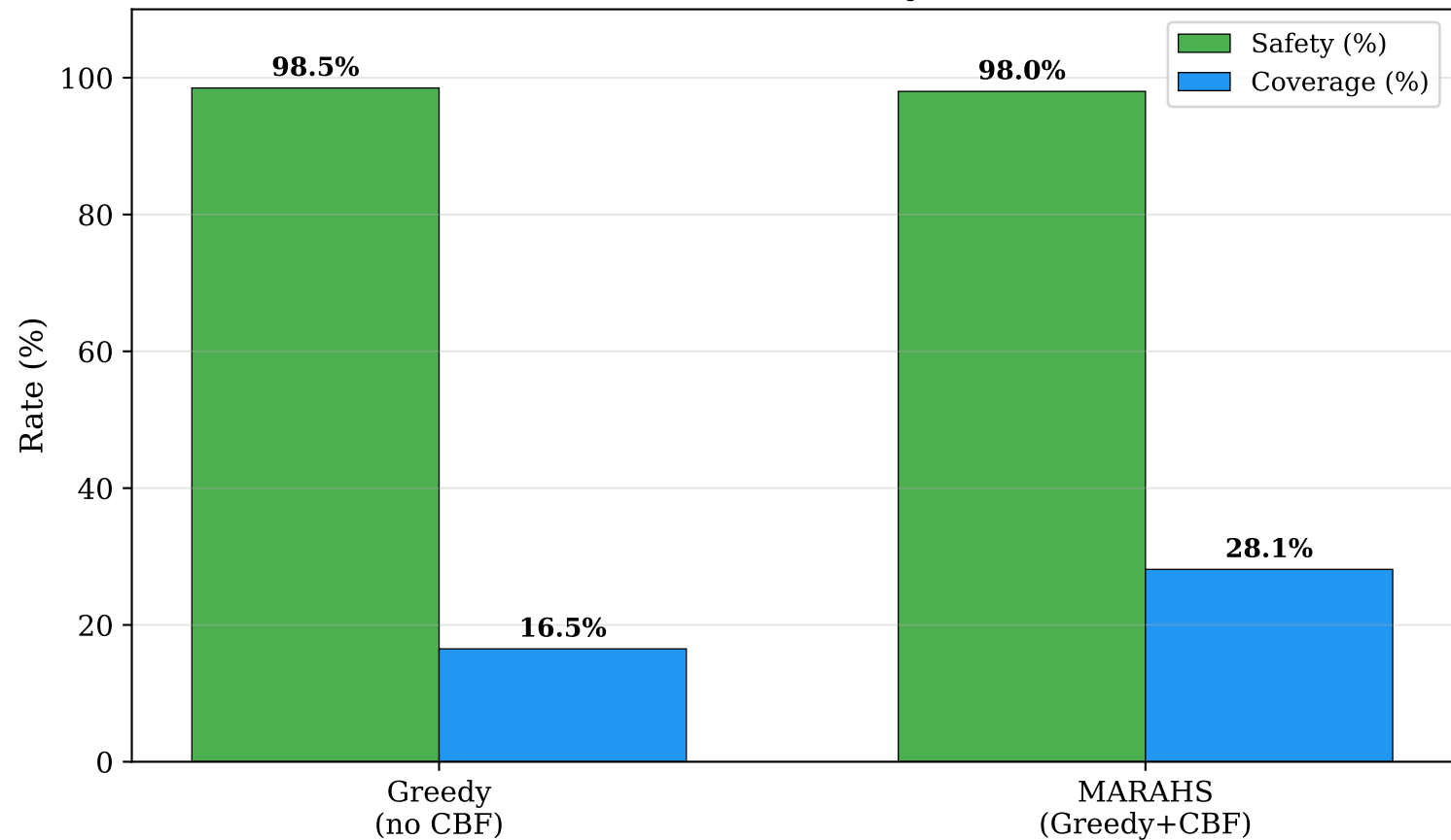
Effect of CBF Safety Filter
