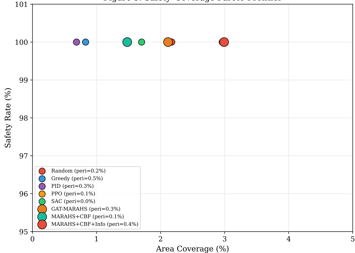
Figure 3: Safety-Coverage Pareto Frontier
