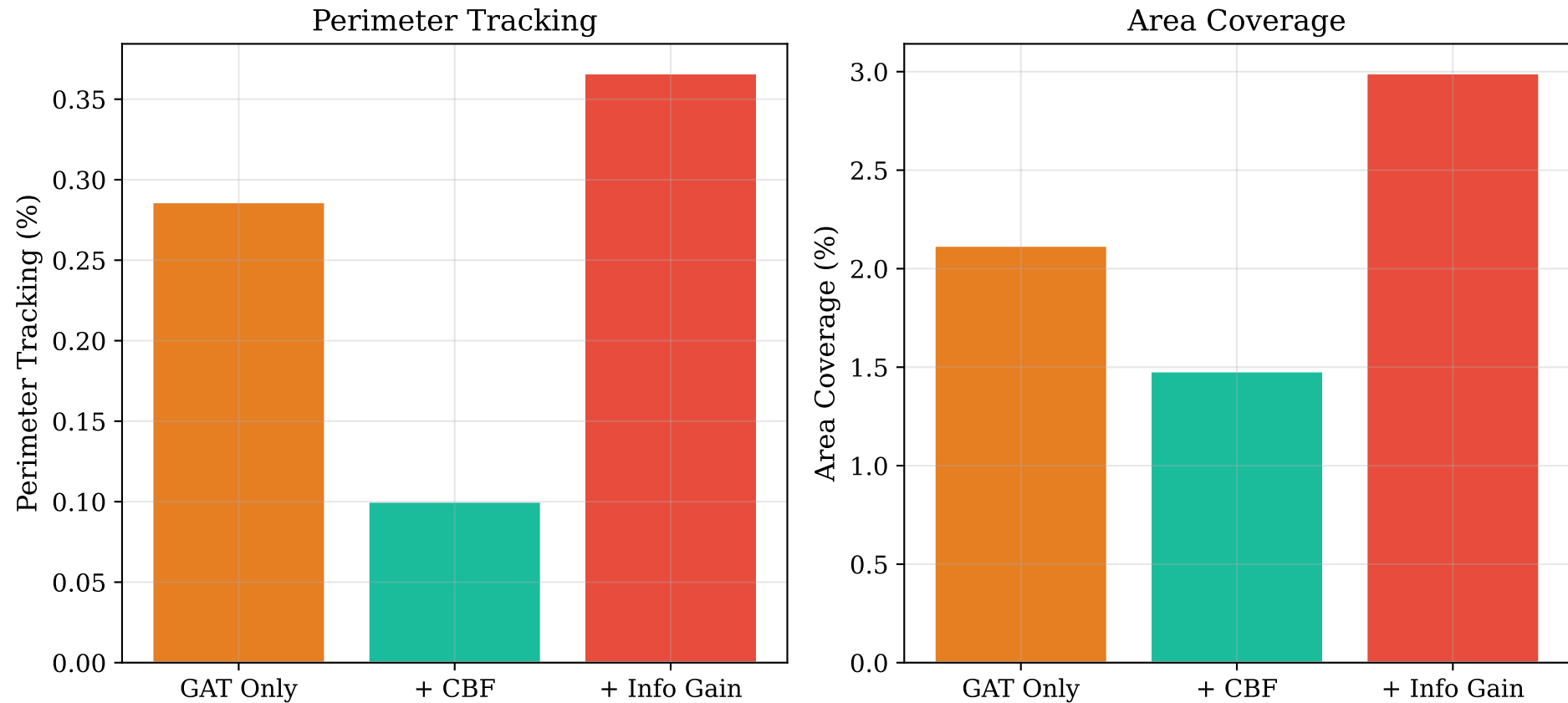
Figure 6: Component Ablation Study
