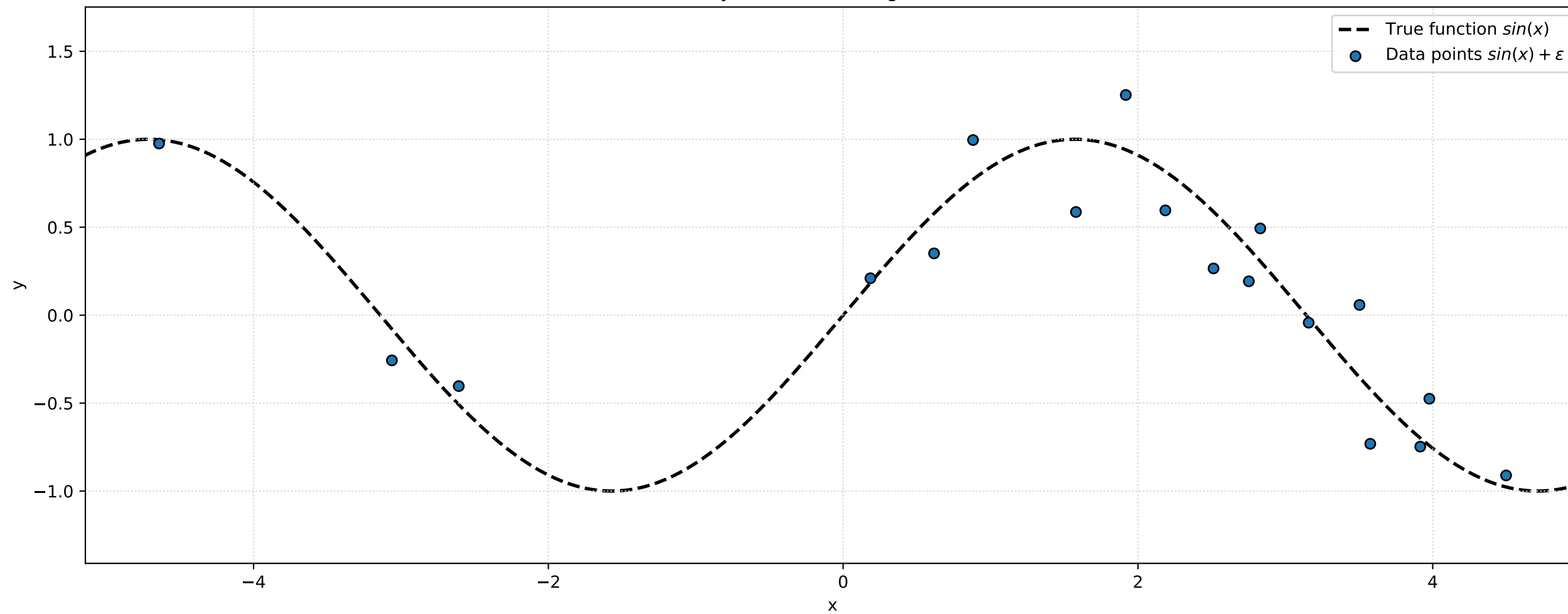
Bayesian Linear Regression
