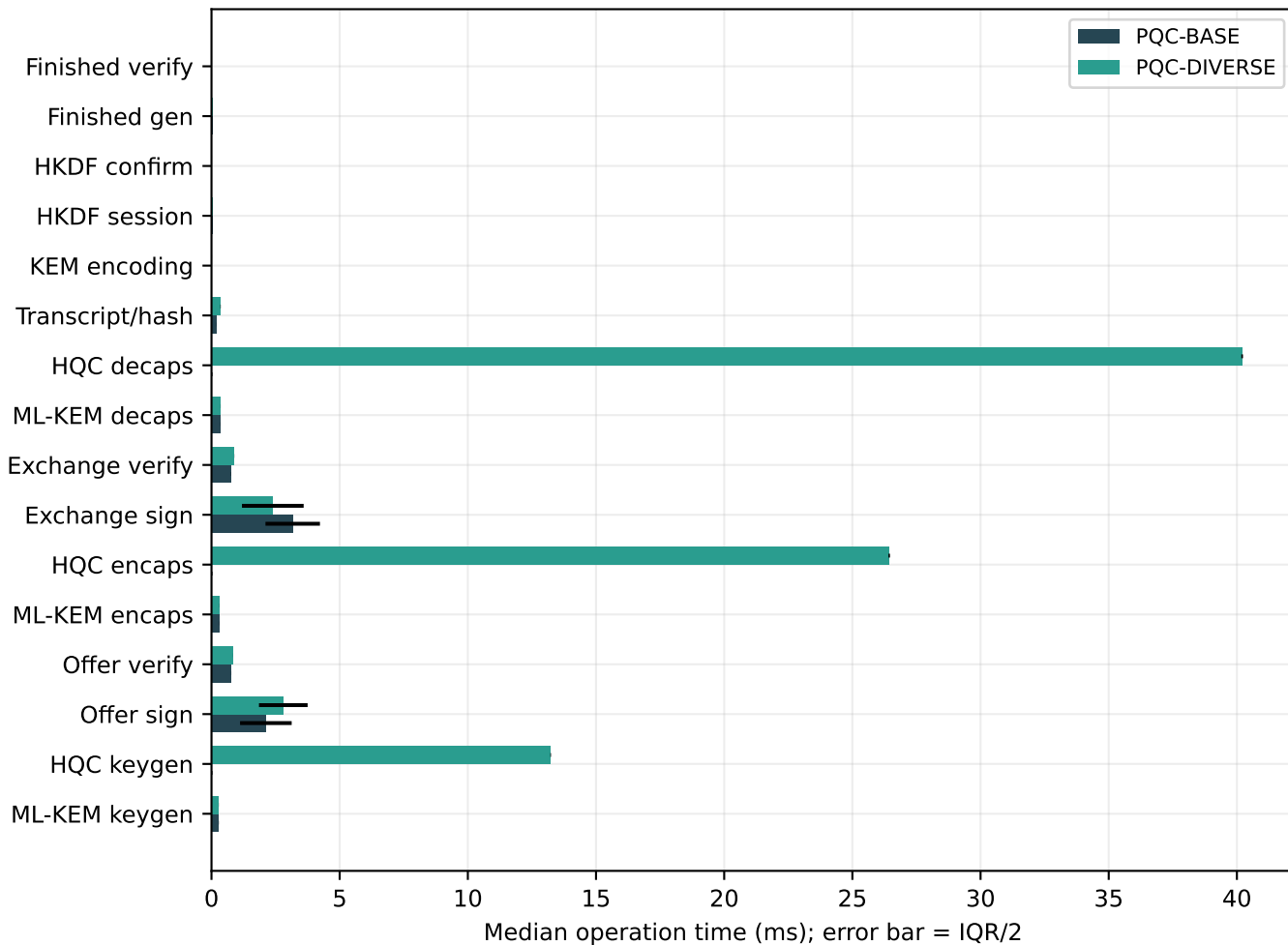
E1 exact PQC operation timings
