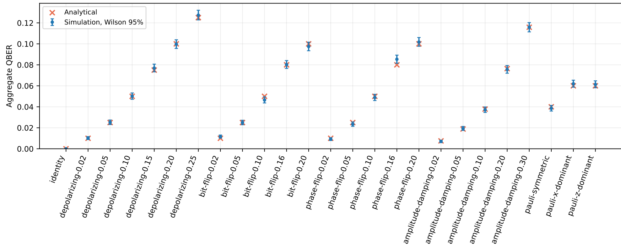
E2 analytical model vs numerical simulation
