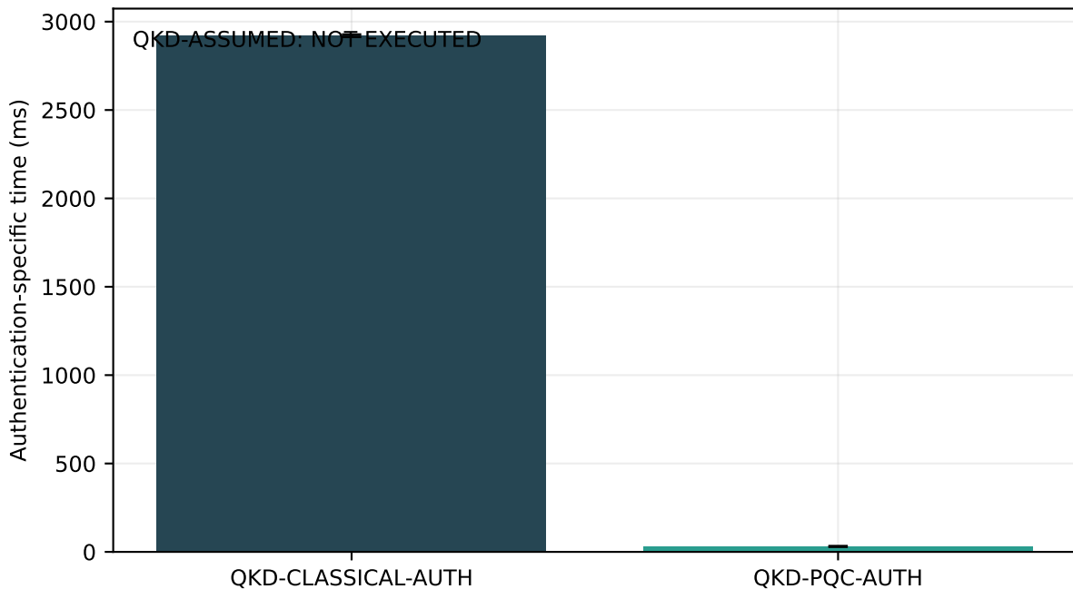
E4 executed authentication software cost
