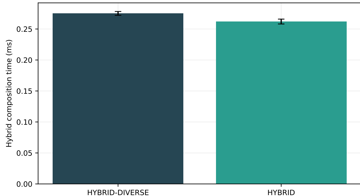
E5 local composition cost (excludes BB84 simulation)
