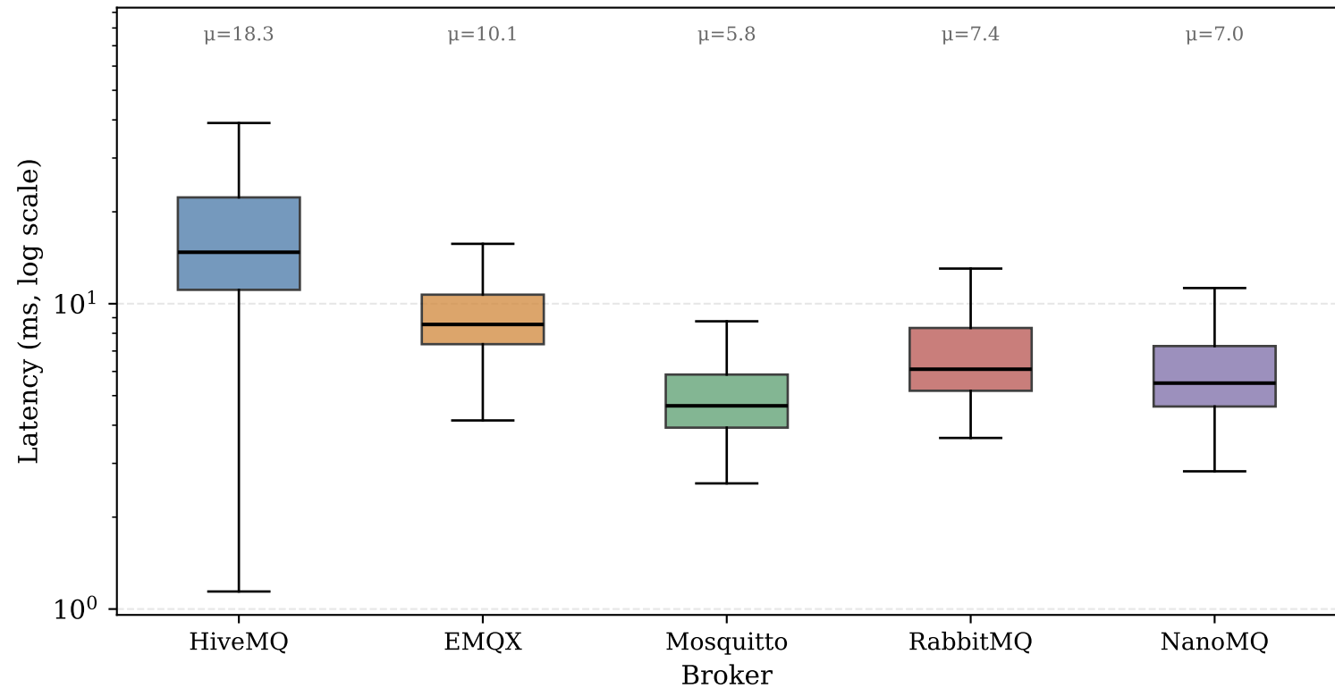
End-to-End Latency — 125 KB Payload (QoS 0)
