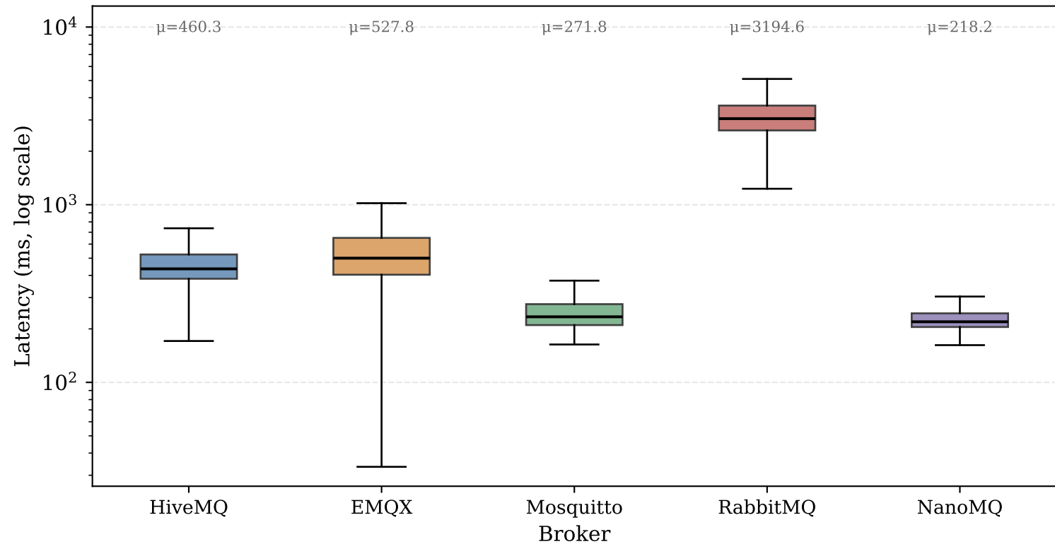
End-to-End Latency — 16 MB Payload (QoS 0)
